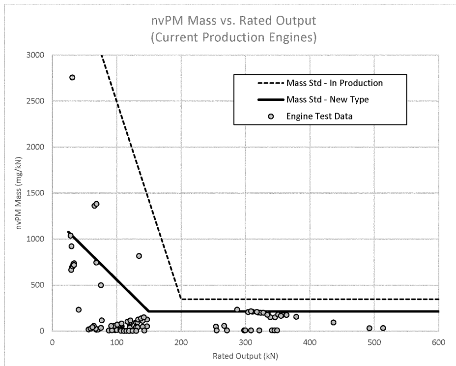
Figure IV-1 - nvPM mass standards compared to in-production engine LTO emission rates
