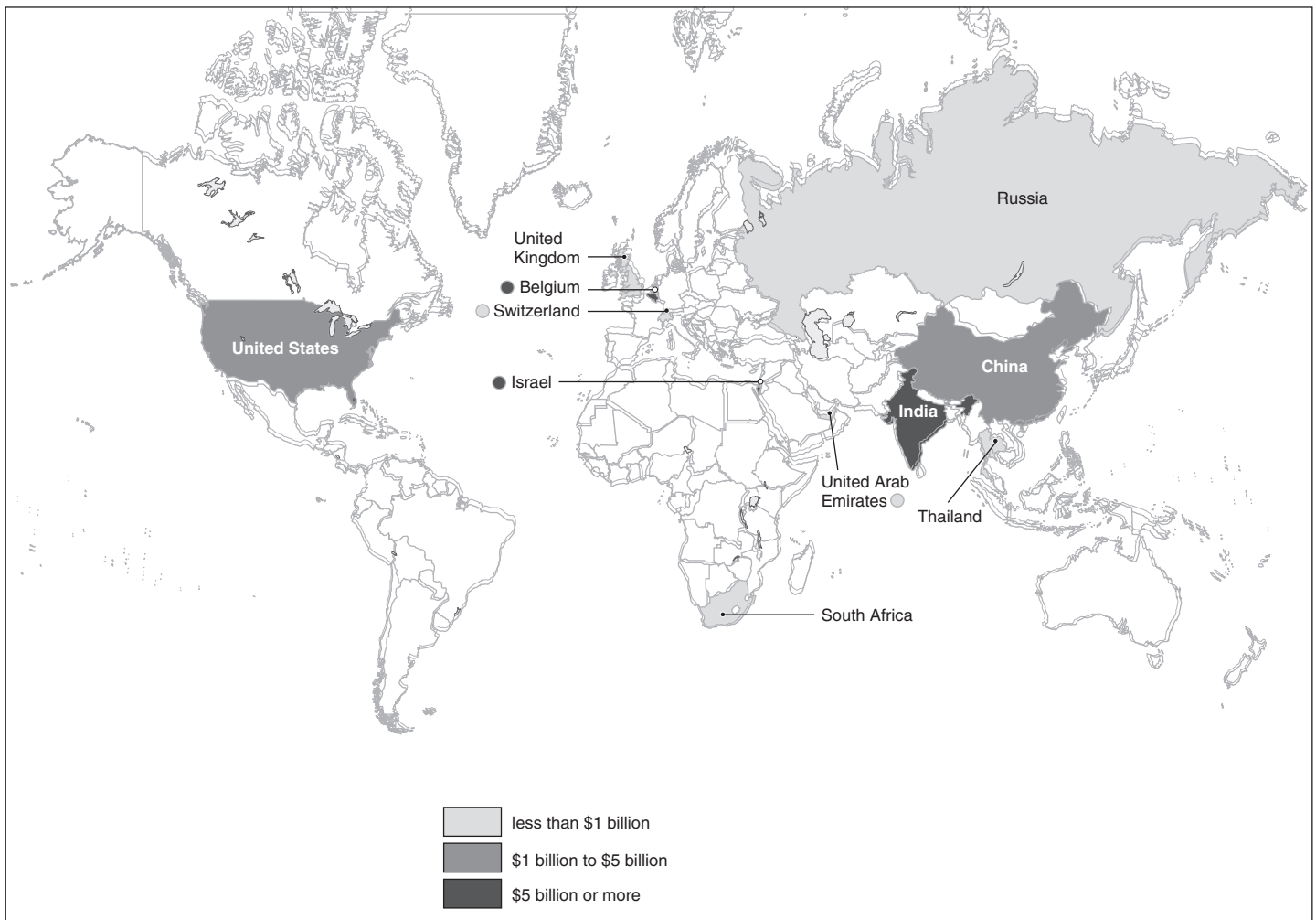
Figure 7: Top Polished Diamond Exporting Countries, 2004 (estimated exports > $200 million)
