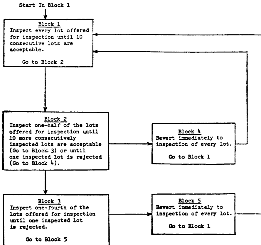
§ 42.123 Flow diagram for skip lot sampling and inspection.
