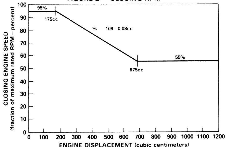
FIGURE 2 – CLOSING RPM
