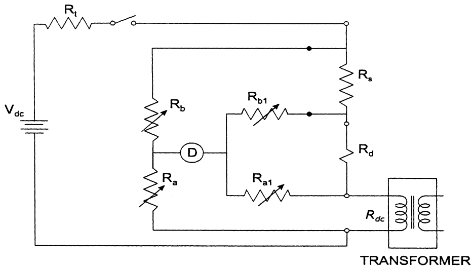
Figure 3.2 Kelvin Bridge
