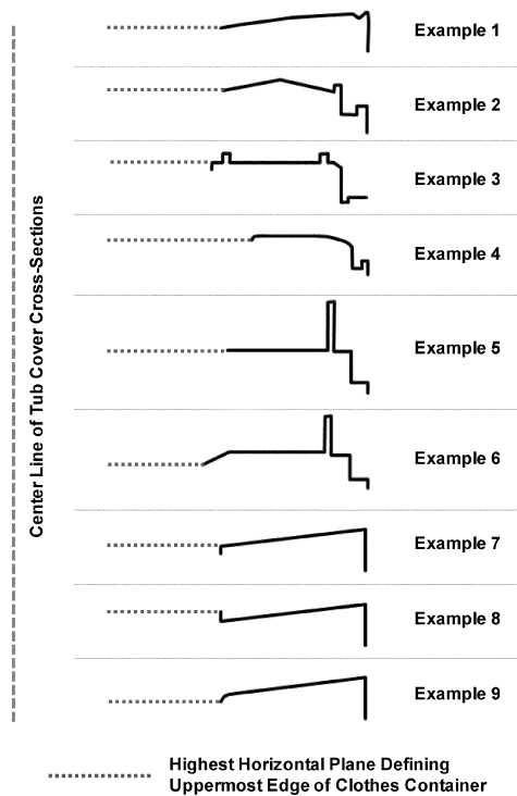
Figure 3.1.4.2— Example Cross-Sections of Tub Covers Showing the Highest
