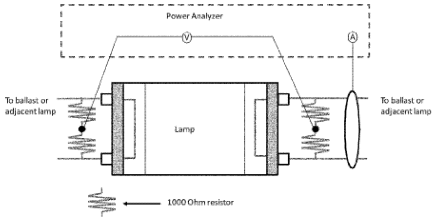
Figure 1: Programmed- and Rapid-Start Ballast Instrumentation Setup
