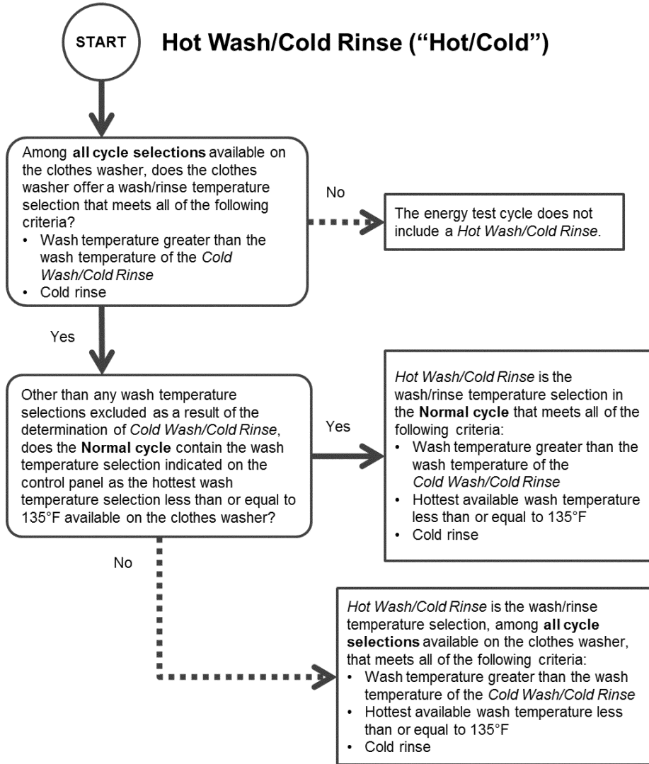
Figure 2.12.2—Determination of Hot Wash/Cold Rinse
