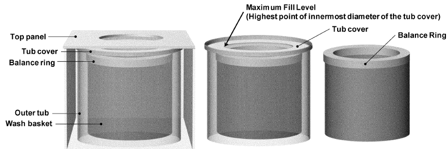
Figure 3.1.4.2— Example Cross-Sections of Tub Covers Showing the Highest
