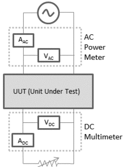
Figure 1. Example Connection Diagram for EPS Efficiency Measurements
