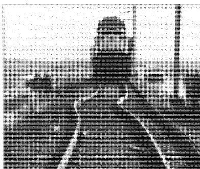
Figure 2-9. Rail Thermal Misalignment 135
