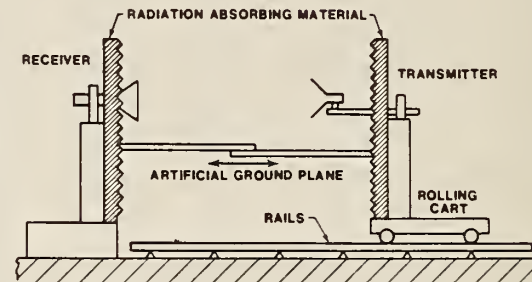
Fig. 1. Schematic diagram showing the NBS indoor extrapolation range modified to function as a scaled model of the larger outdoor range.
