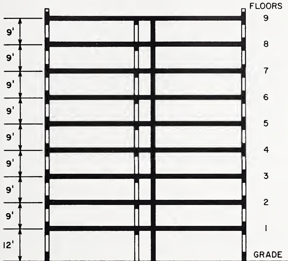
FIGURE 3 - BUILDING CROSS-SECTION AND WALL THICKNESSES
