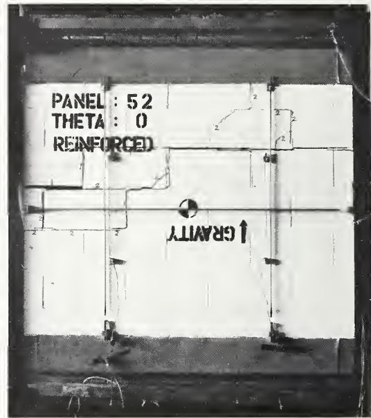
Fig. 23 Multiple Cracking of Reinforced Panel.
