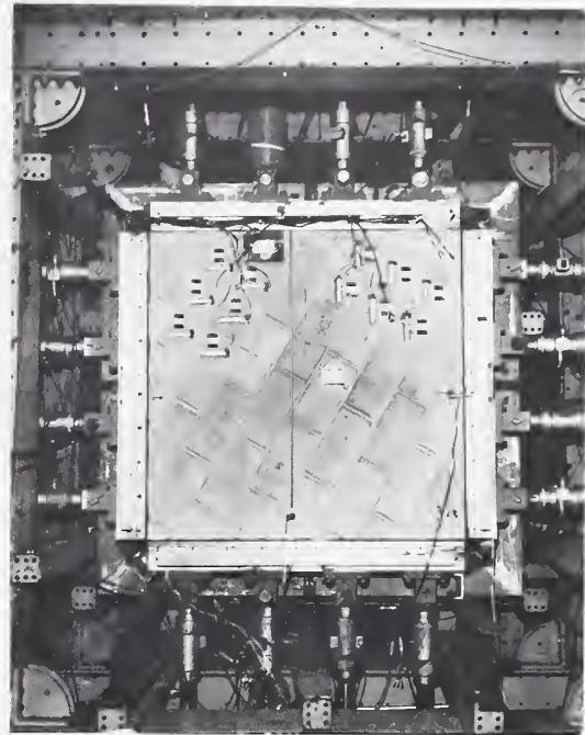
Fig. 4 Biaxial Fixture.
