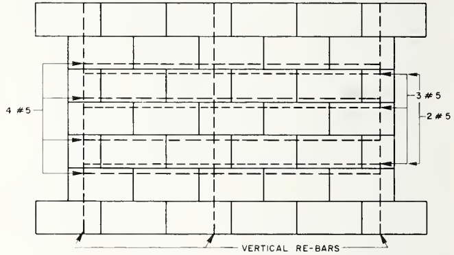
REINFORCEMENT DETAILS FOR HOLLOW CONCRETE BLOCK WALLS - 3'-4" x 6' x 8"
