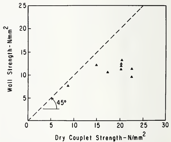
Fig. 25 Comparison of UngROUTED Wall and Couplet Strengths.
