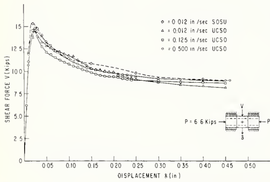
Fig. 30 Strain-Rate Dependence.
