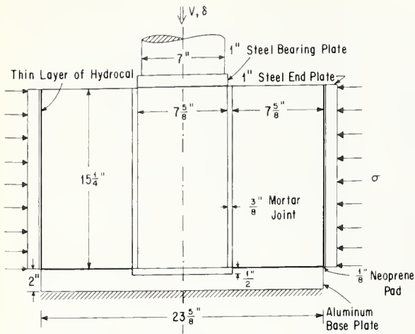
Fig. 28 Joint Test Setup.
