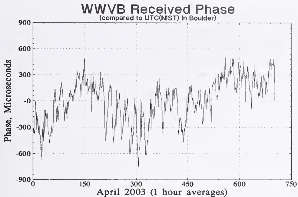
Figure 5.14. WWVB received carrier phase data for April 2003.
