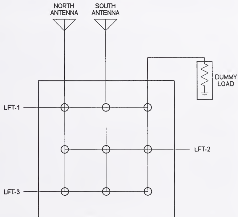
Figure 2.16. RF switch matrix for WWVB transmitters.
