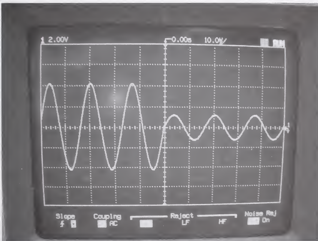
Figure 5.9. WWVB OTM.
