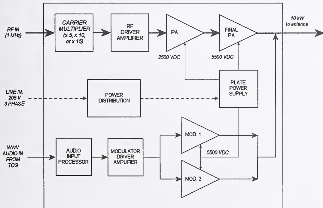
Figure 2.9. Block diagram of a CCA transmitter.
