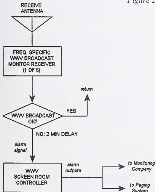
Figure 2.13. WWV monitoring and alarm system.
