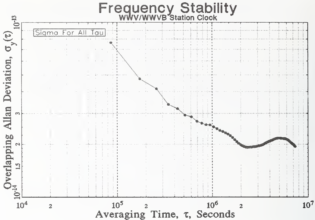
Figure 5.4. Estimated frequency stability of WWV/WWVB station clock.
