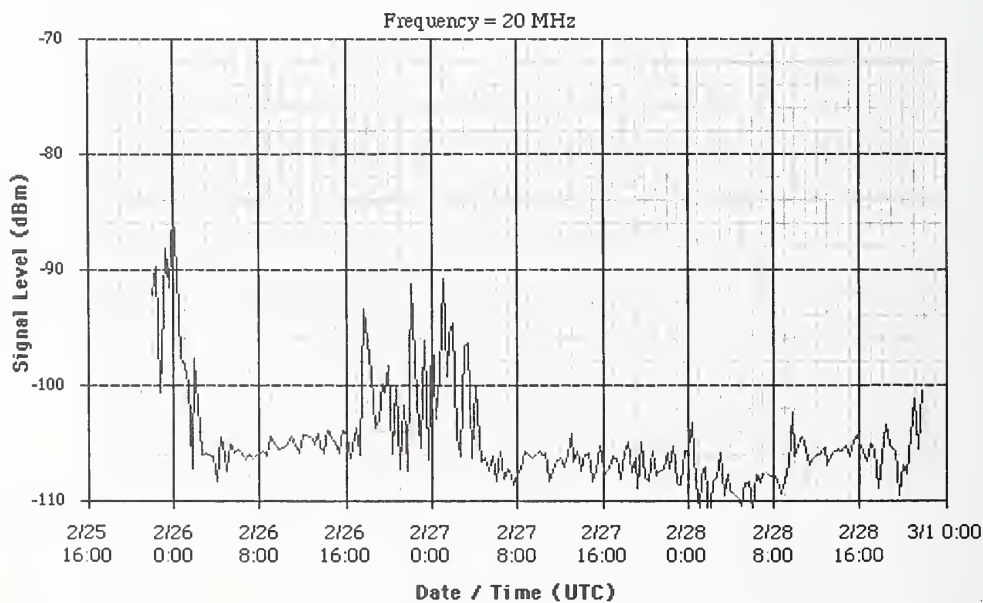
Figure 4.2. Sample graphs of WWV/WWVH field strength as recorded by HAARP in Gakona, Alaska.
