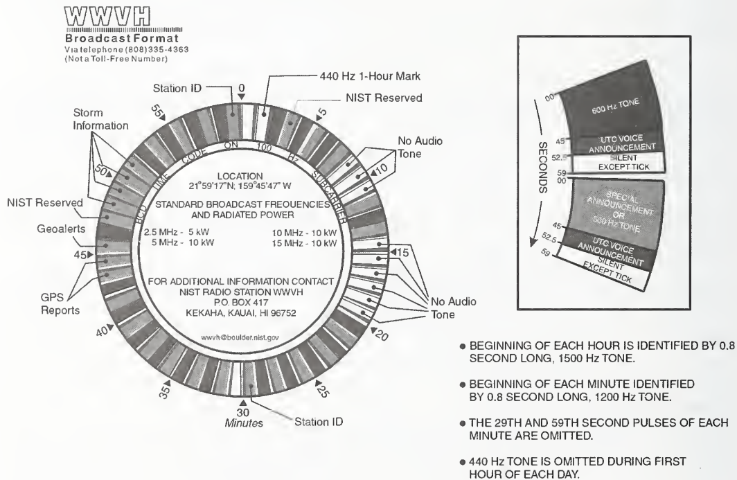
Figure 2.23. WWVH audio broadcast format.
