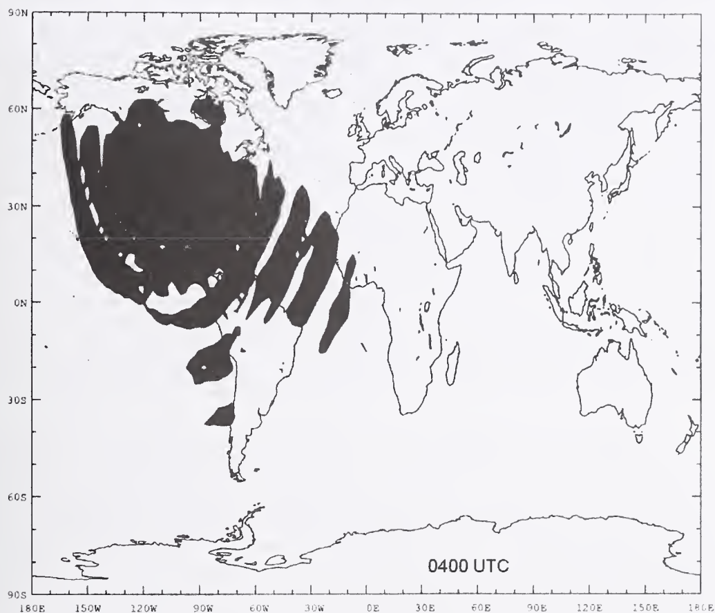
Figure 4.4. Predicted WWVB coverage at 0400 UTC (night).
