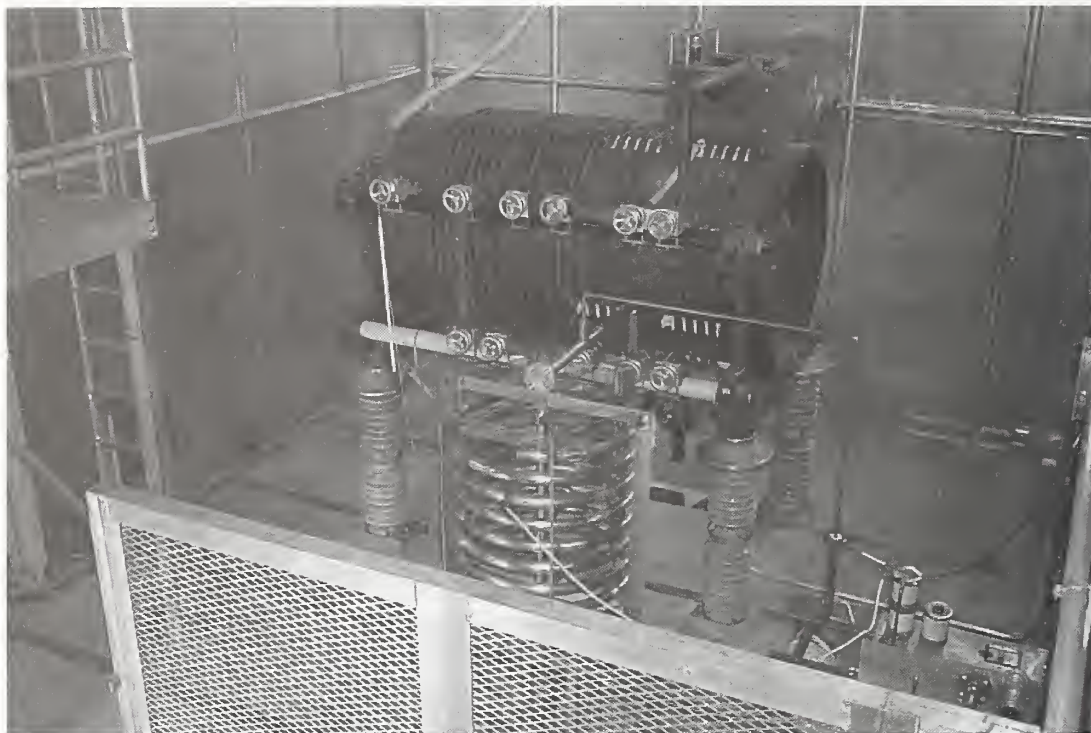
Figure 2.18. Interior view of helix house.
