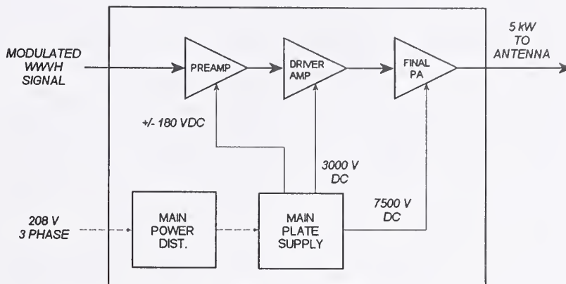
Figure 2.24. Simplified block diagram of modified AEL transmitter.
