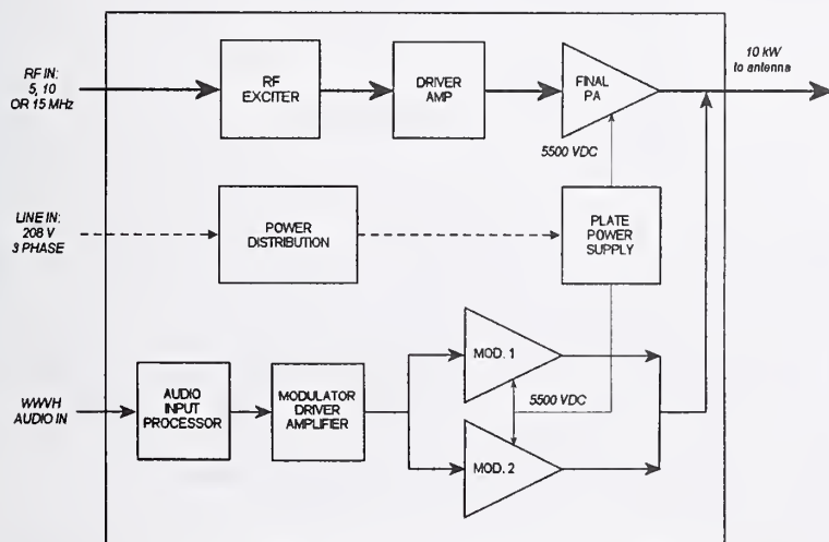
Figure 2.25. Simplified block diagram of Elcom-Bauer transmitter.
