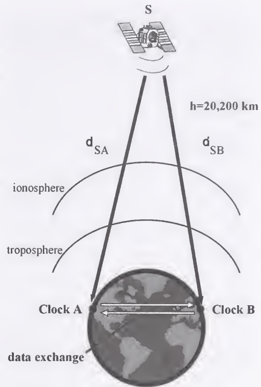
Figure 5.1. Common-view GPS technique.
