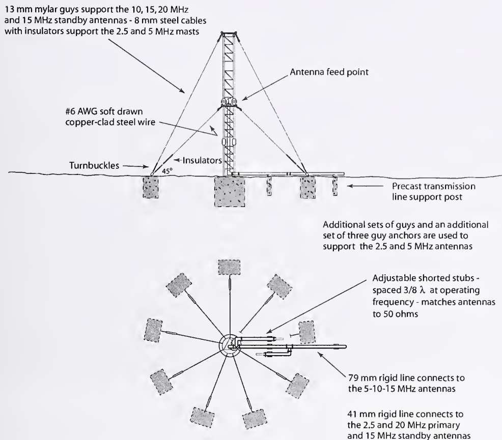
Figure 1.11. WWV primary antenna and tuning stub installation.
