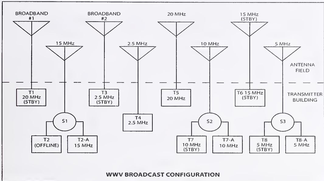
Figure 1.9. Transmitter/antenna connections at WWV.
