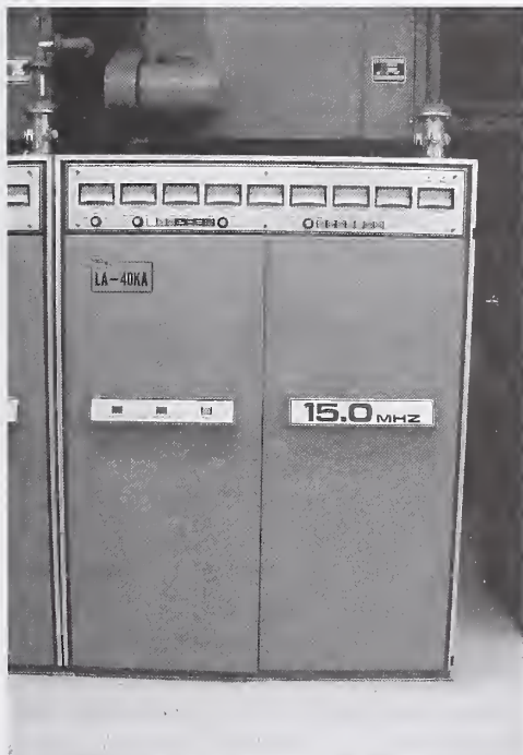
Figure 1.26. The 15 MHz standby transmitter at WWVH.
