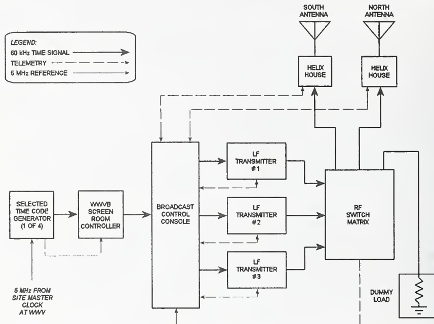
Figure 1.17. WWVB broadcast equipment configuration.
