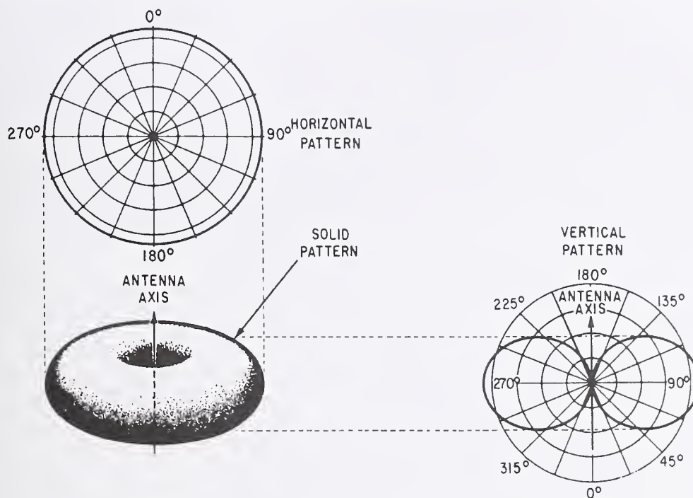
Figure 2.10. Theoretical radiation pattern of ideal vertical half-wave dipole antenna.
