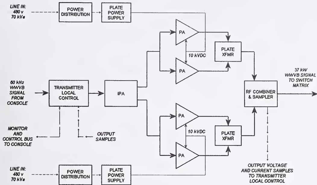
Figure 2.17. Block diagram of WWVB transmitter.
