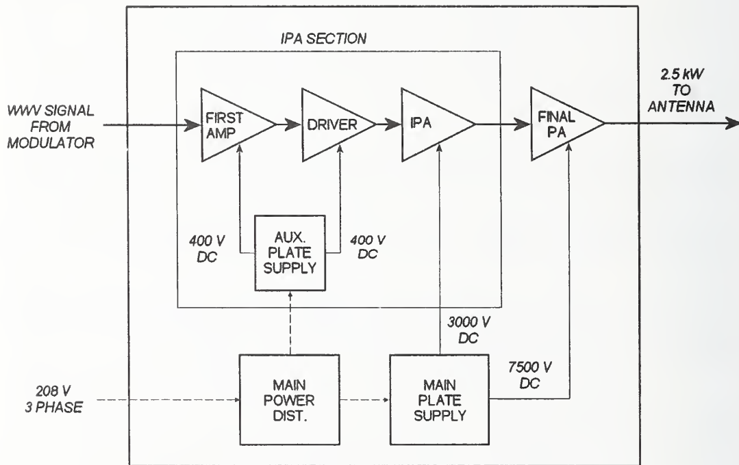
Figure 2.8. Block diagram of a TMC transmitter.
