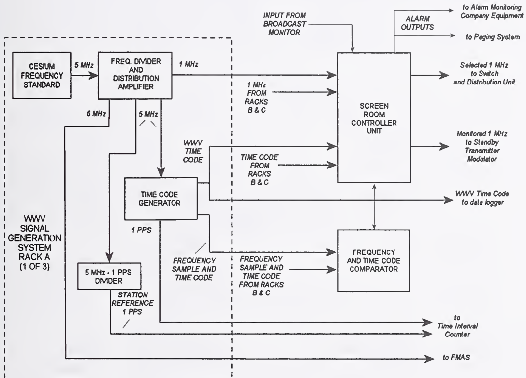
Figure 2.2. WWV broadcast equipment rack.
