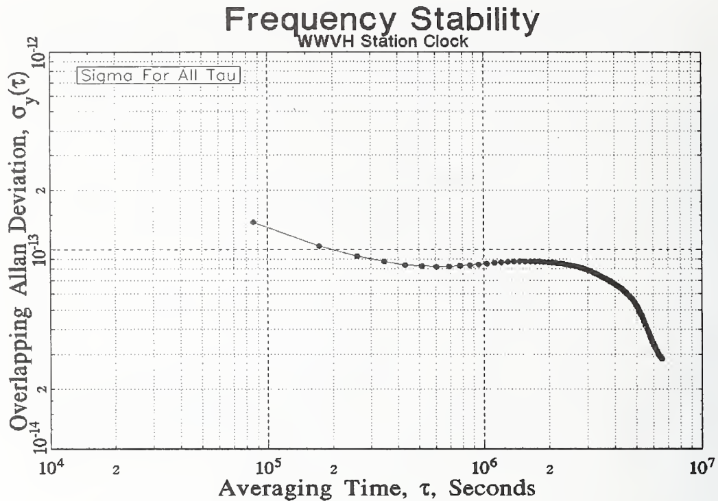
Figure 5.6. Estimated frequency stability of WWVH station clock.
