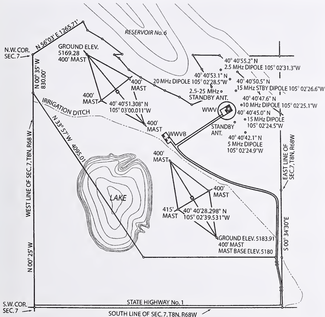
Figure 1.4. WWV and WWVB site map.
