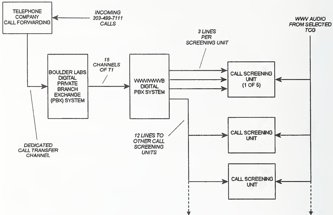
Figure 2.27. Block diagram of WWV Telephone Time-of-Day System.
