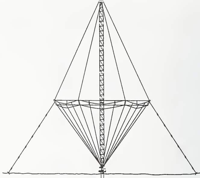
Figure 1.12. Broadband monopole antenna at WWV.
