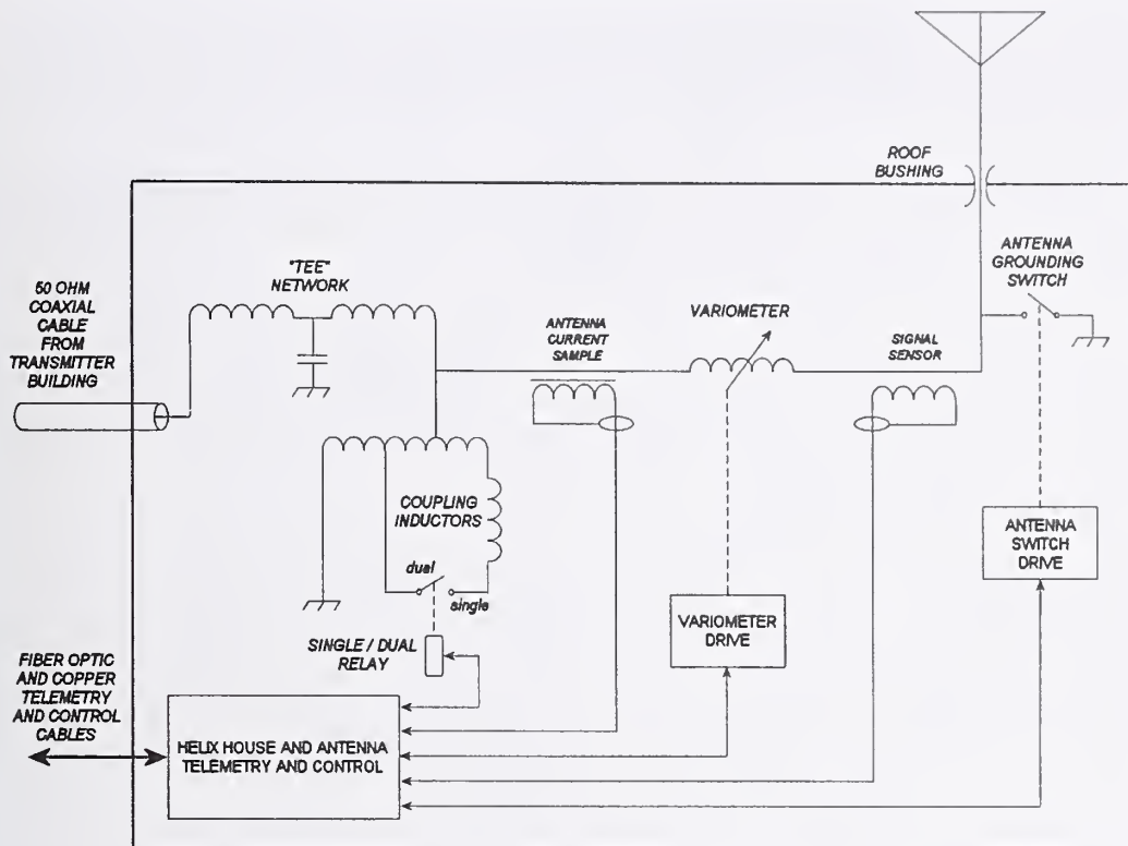
Figure 2.19. Simplified diagram of WWVB helix house.
