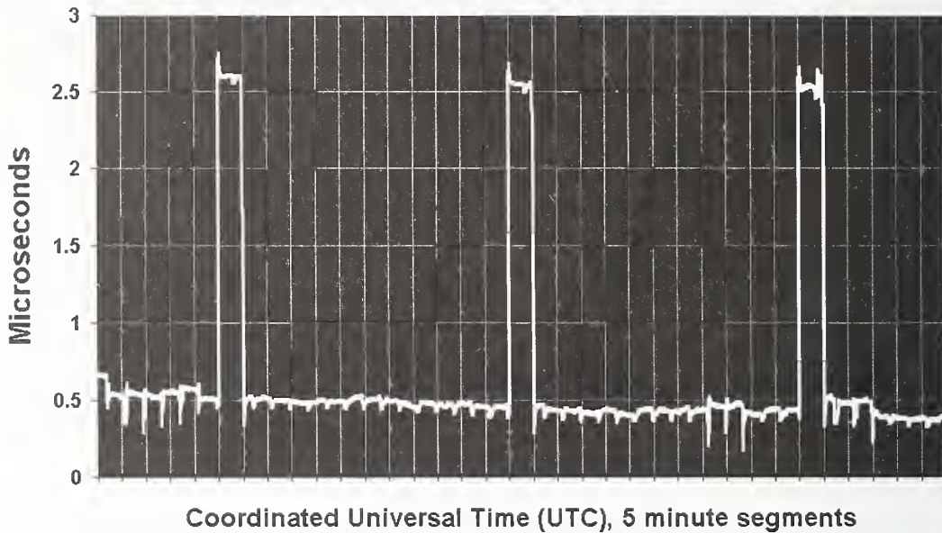
Figure 2.14. WWVB phase signature.
