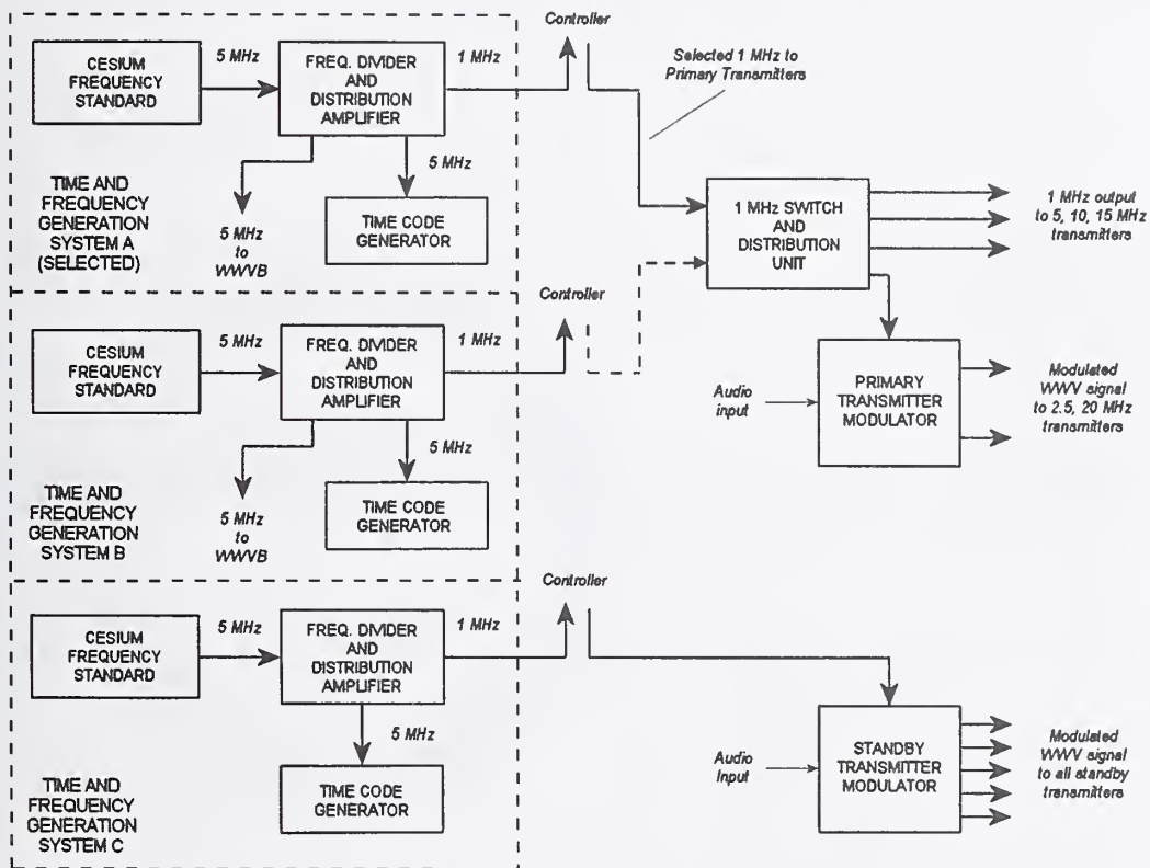
Figure 2.4. WWV standard carrier frequency generation system.
