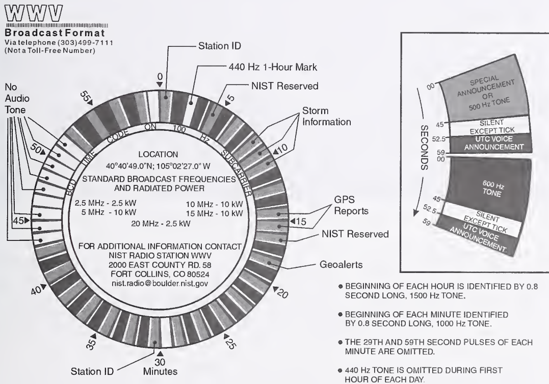
Figure 2.5. WWV audio broadcast format.
