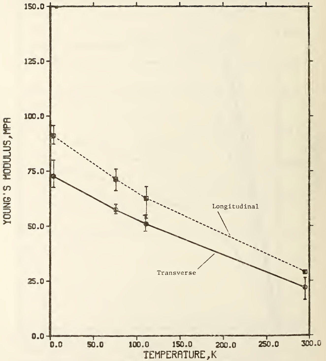
Figure 34. Compressive Young's modulus versus temperature for a 96-kg/m 3 polyurethane foam.
