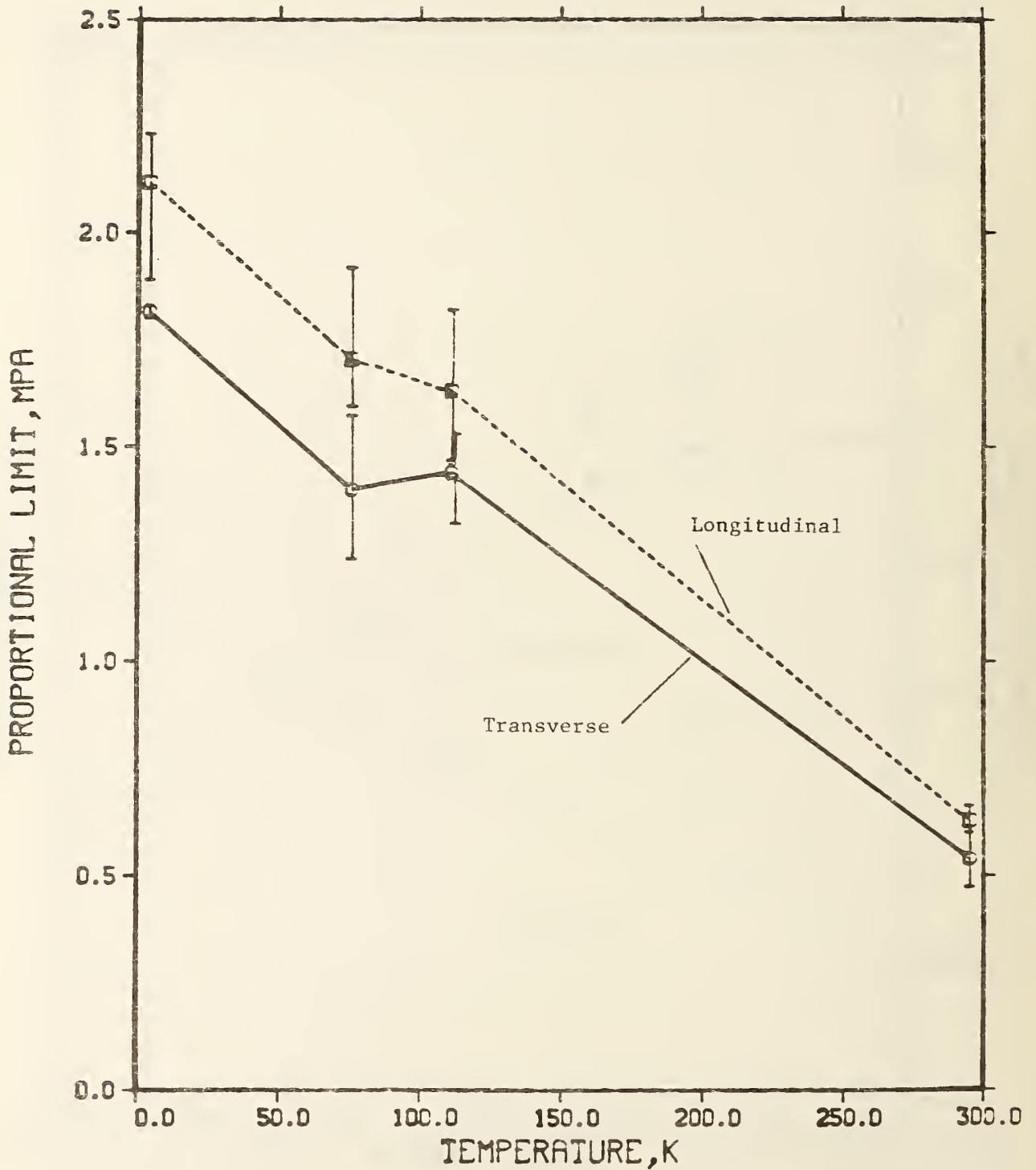
Figure 36. Compressive proportional limit versus temperature for a 96-kg/m 3 polyurethane foam.
