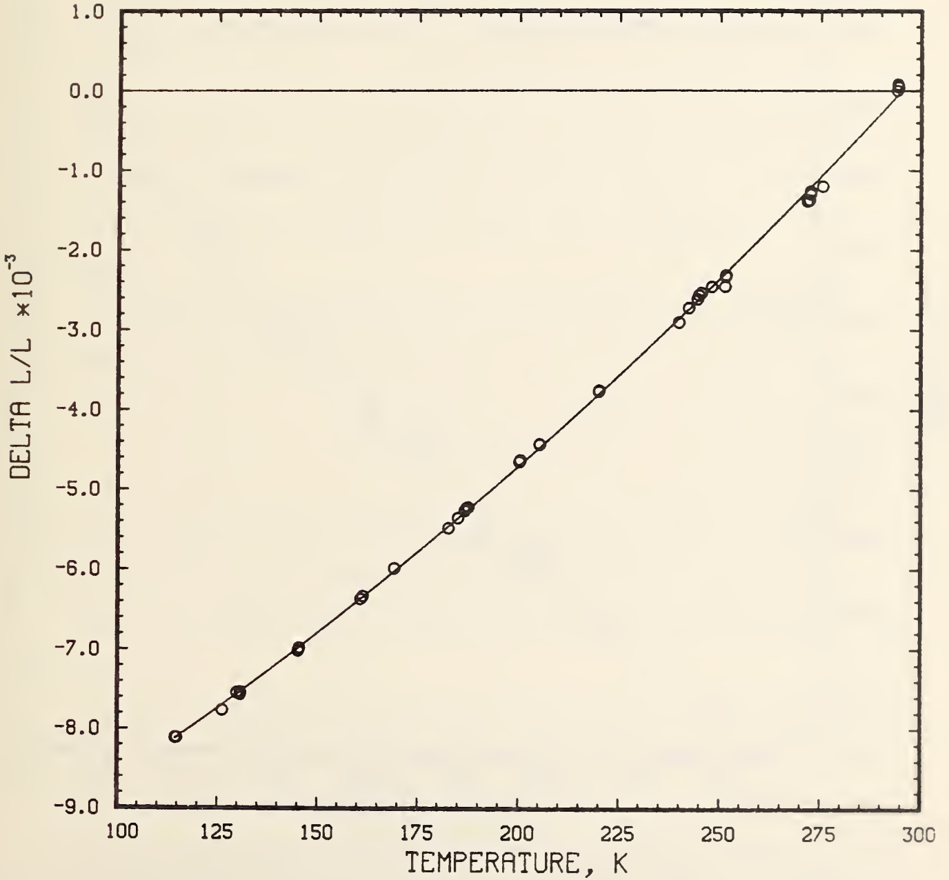
Figure 11. Thermal expansion of a 54-kg/m 3 polyurethane foam specimen. Experimental data are represented by discrete points and the solid line represents a three-term polynomial fit to these data. The reference temperature is 295.180 K
