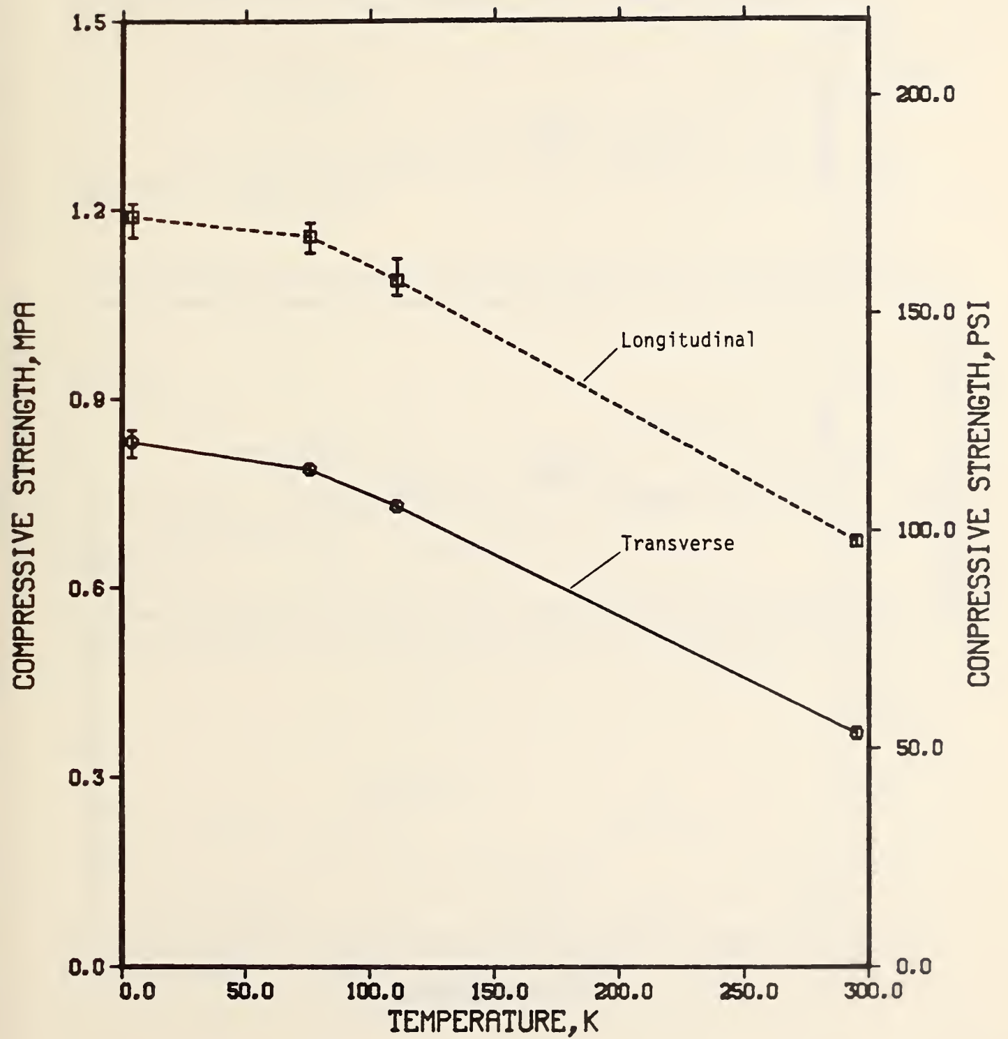
Figure 27. Compressive strength versus temperature for a 64-kg/m 3 polyurethane foam.
