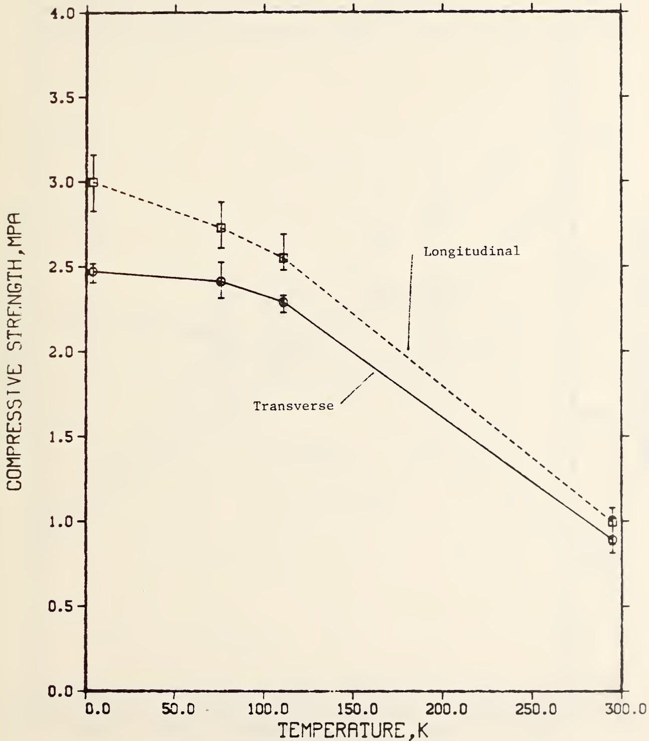
Figure 35. Compressive strength versus temperature for a 96-kg/m 3 polyurethane foam.
