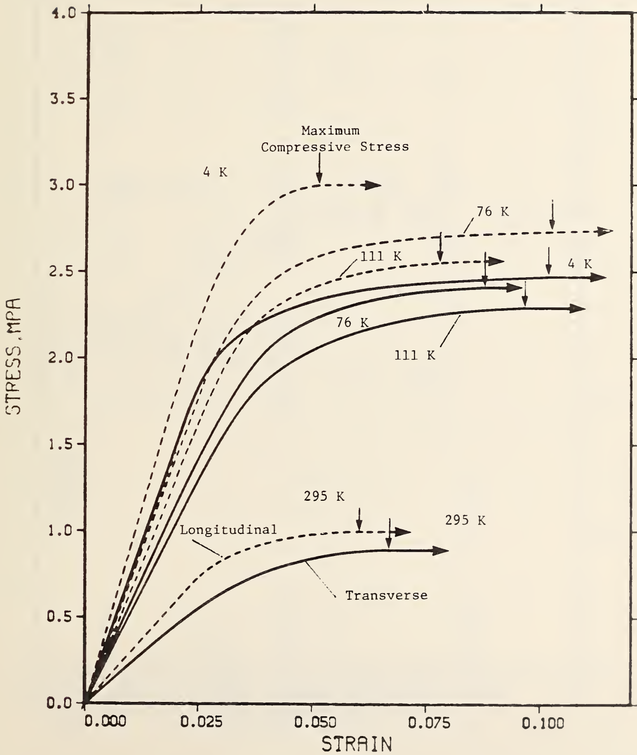
Figure 39. Compressive stress versus strain for a 96-kg/m 3 polyurethane foam.
