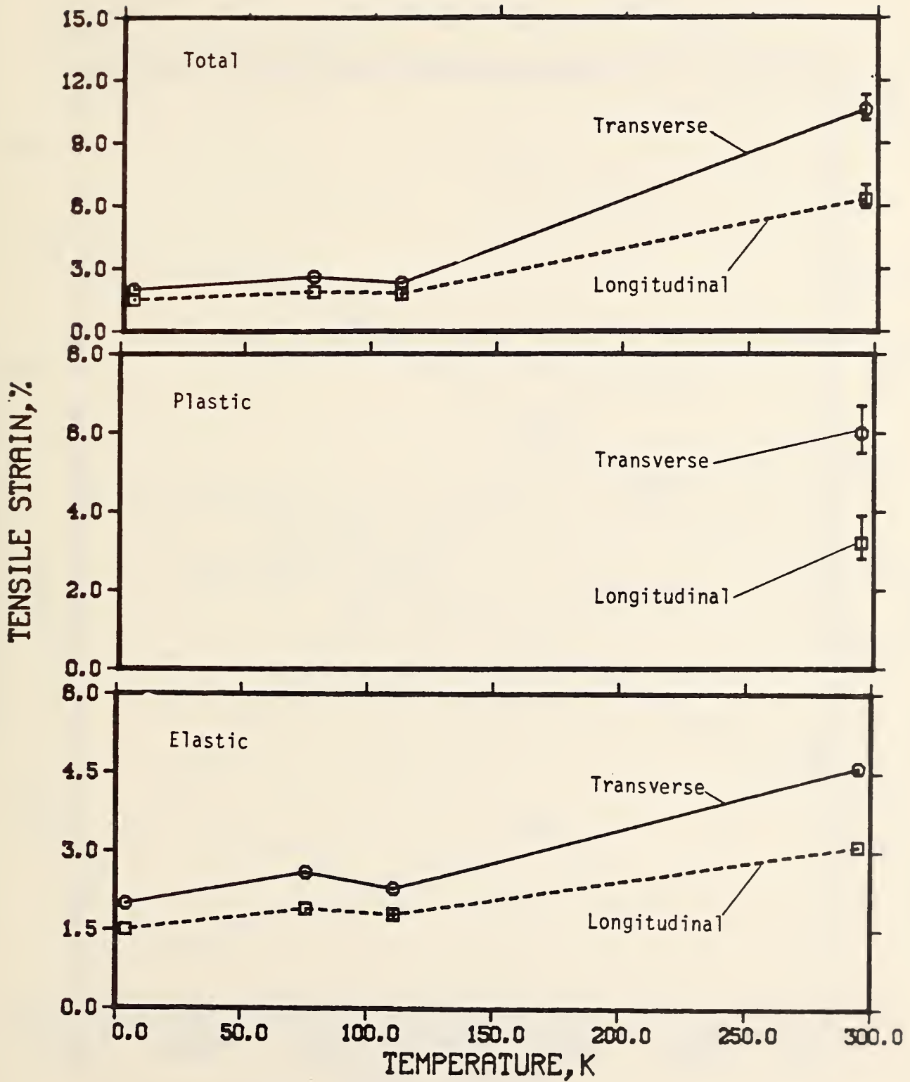
Figure 25. Tensile strain versus temperature for a 64-kg/m 3 polyurethane foam.
