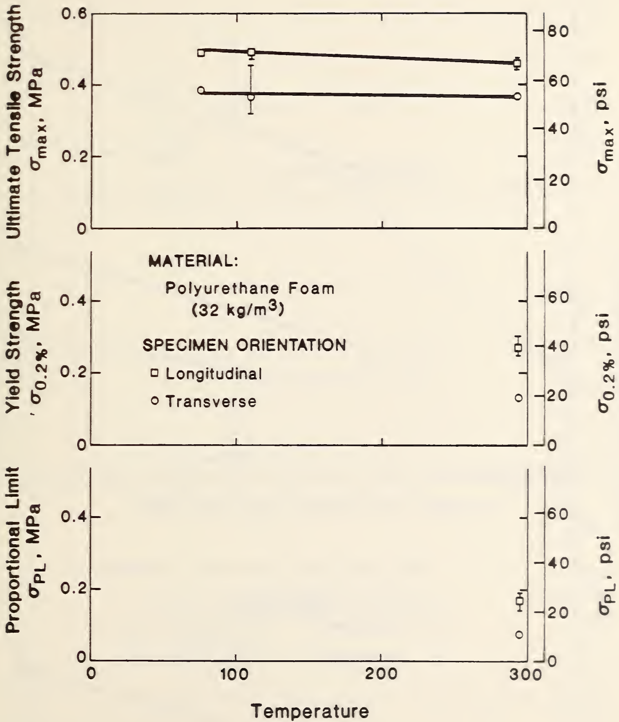
Figure 17. Tensile test results: proportional limit, yield strength, and ultimate strength versus temperature for a 32-kg/m 3 polyurethane foam.
