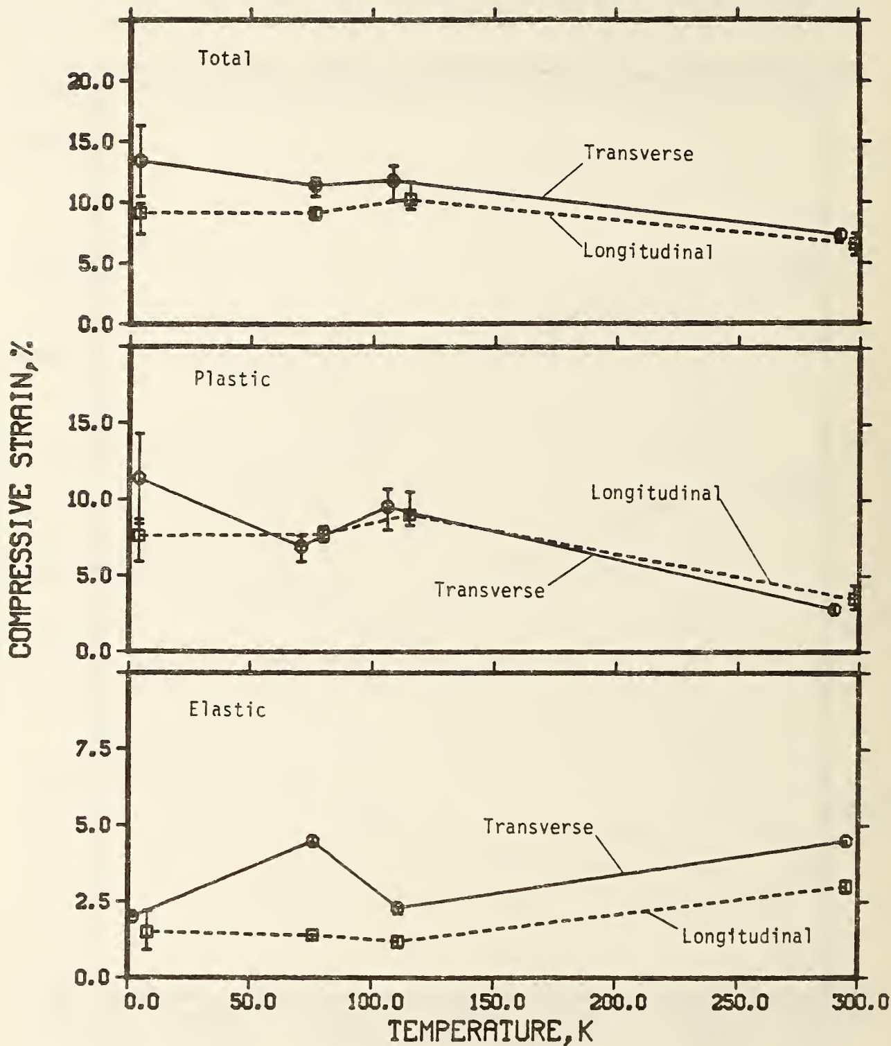
Figure 28. Compressive strain as a function of temperature for a 64-kg/m 3 polyurethane foam.
