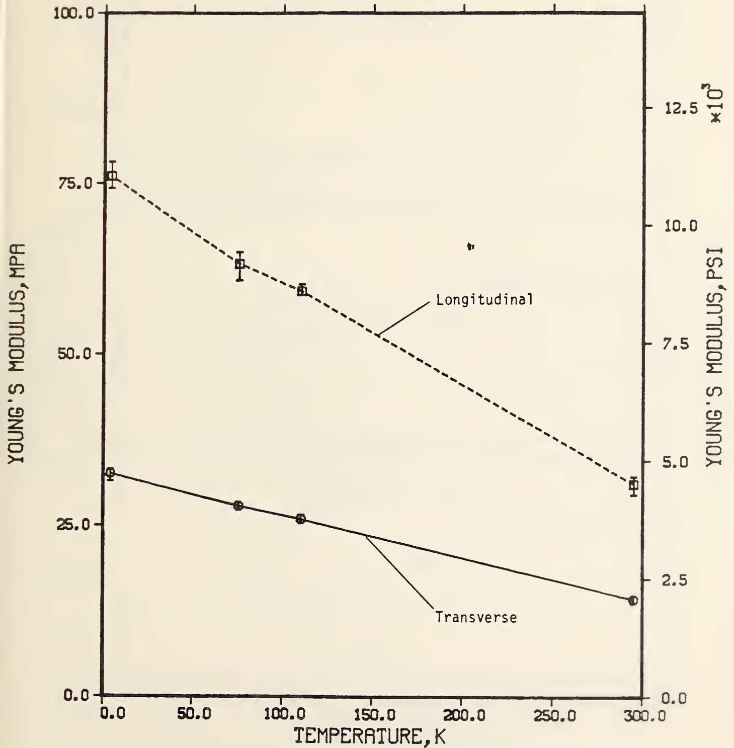
Figure 23. Tensile Young's modulus versus temperature for a 64-kg/m 3 polyurethane foam.
