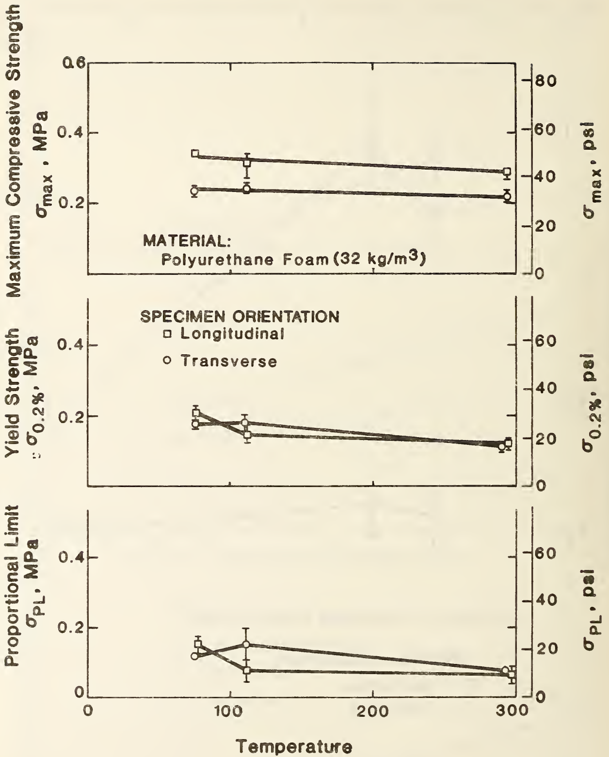
Figure 20. Compression test results: proportional limit, yield strength, and maximum compressive strength versus temperature for a 32-kg/m 3 polyurethane foam.
