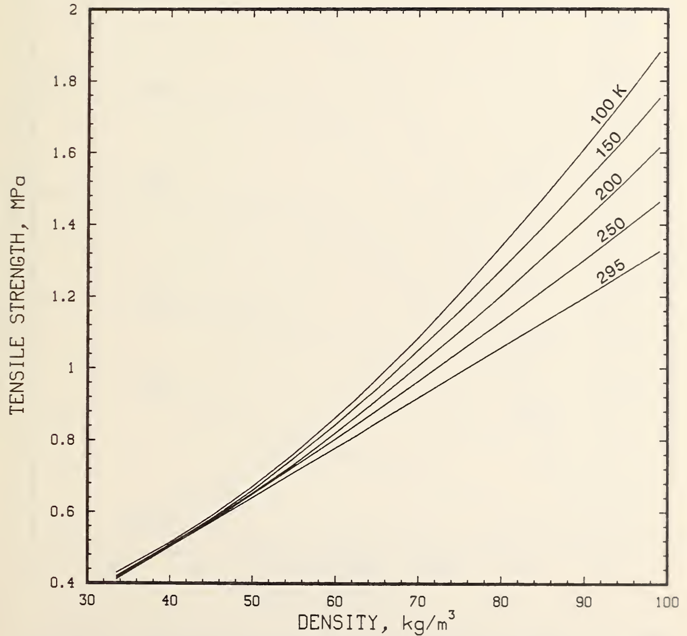
Figure 46. Strength of polyurethane foams in tension as a function of density with temperature as the parameter. Strength obtained here must be modified by a function of (H/W) for a specific material.
