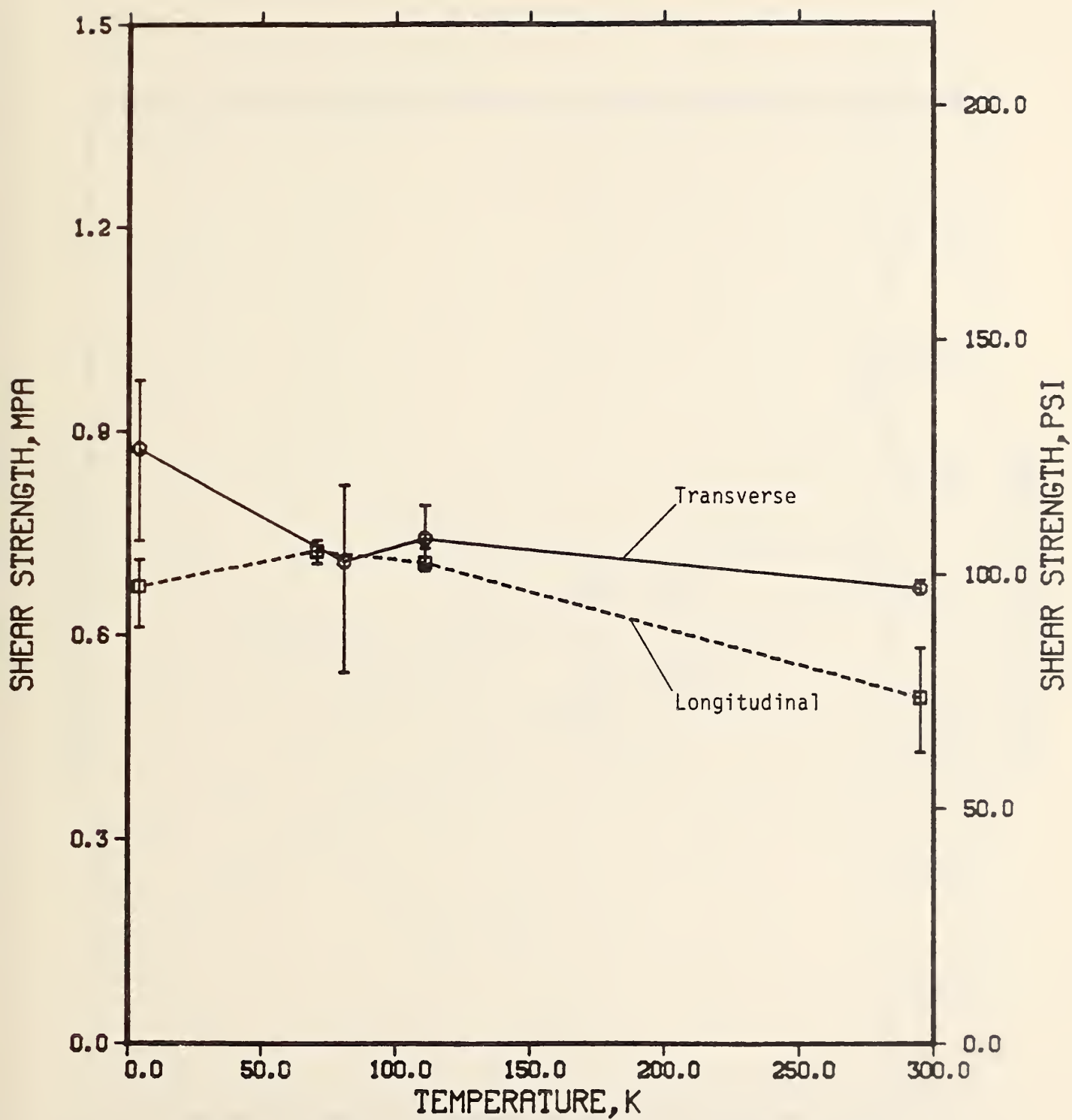
Figure 29. Shear strength versus temperature for a 64-kg/m 3 polyurethane foam.
