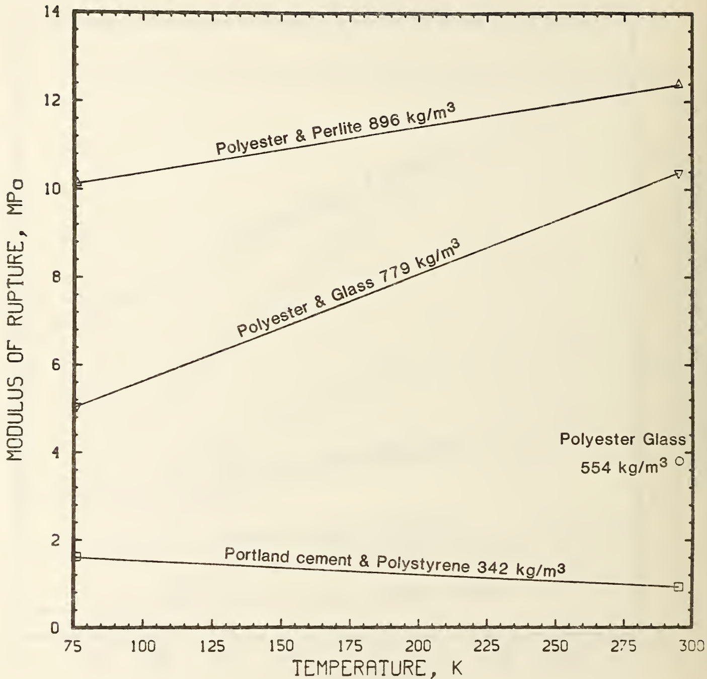
Figure 55. Average modulus of rupture of several insulating concretes as a function of temperature (determined at NBS).
