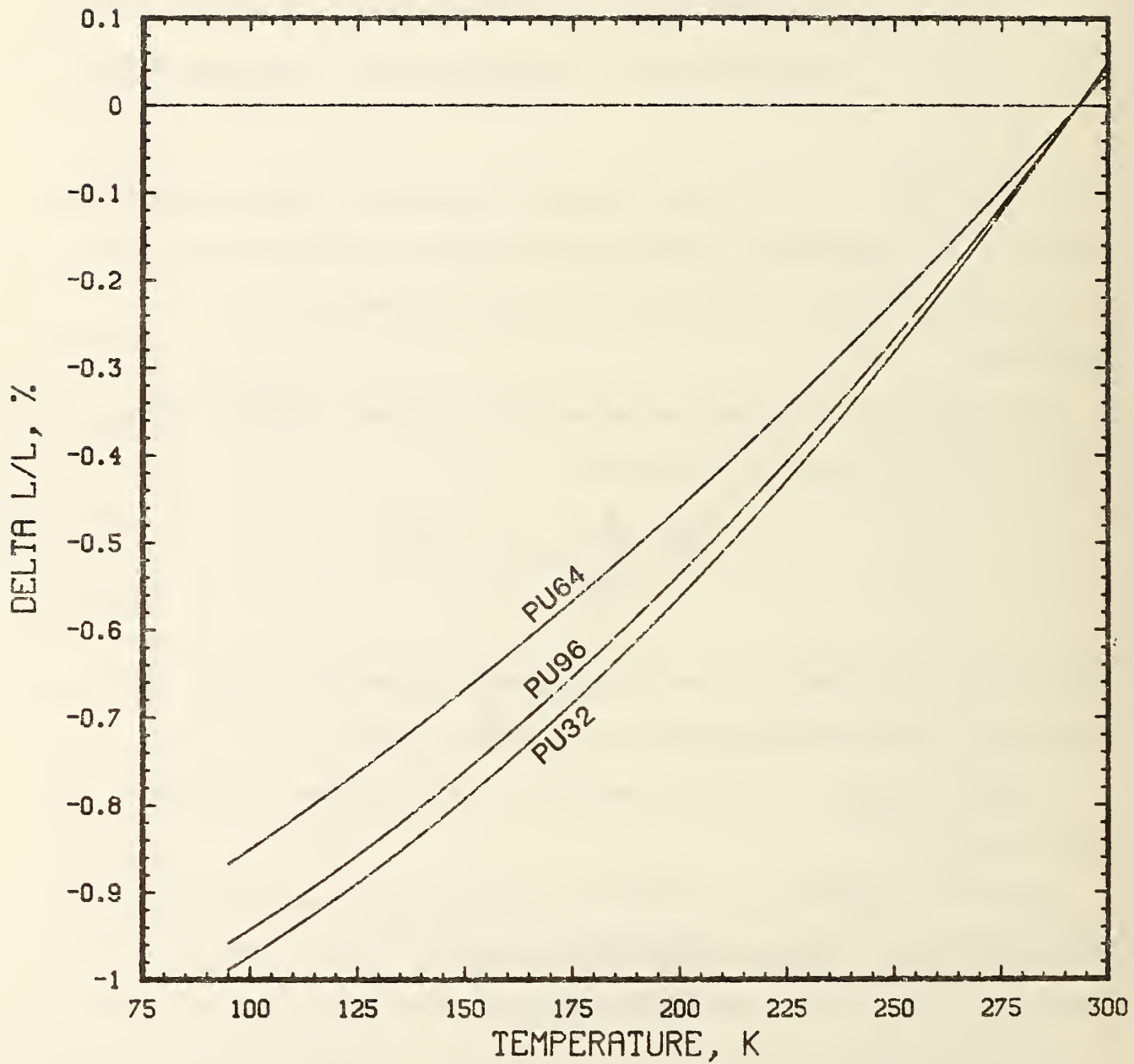
Figure 13. Results of three-term polynomial fits to the thermal expansion of 32-, 64-, and 96-kg/m 3 polyurethane foam specimens. Reference temperature is 293 K.
