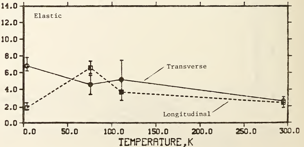
Figure 38. Compressive strain versus temperature for a 96-kg/m 3 polyurethane foam.
