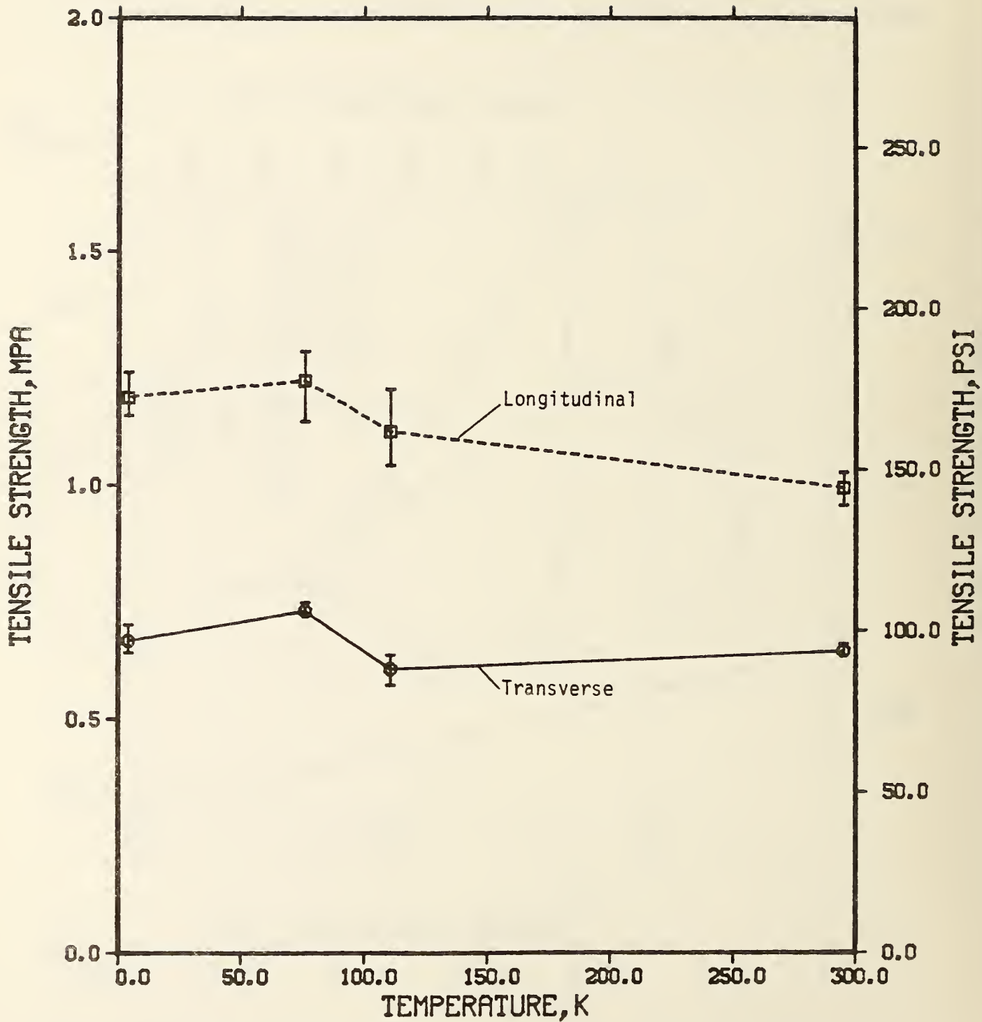
Figure 24. Tensile strength versus temperature for a 64-kg/m 3 polyurethane foam.
