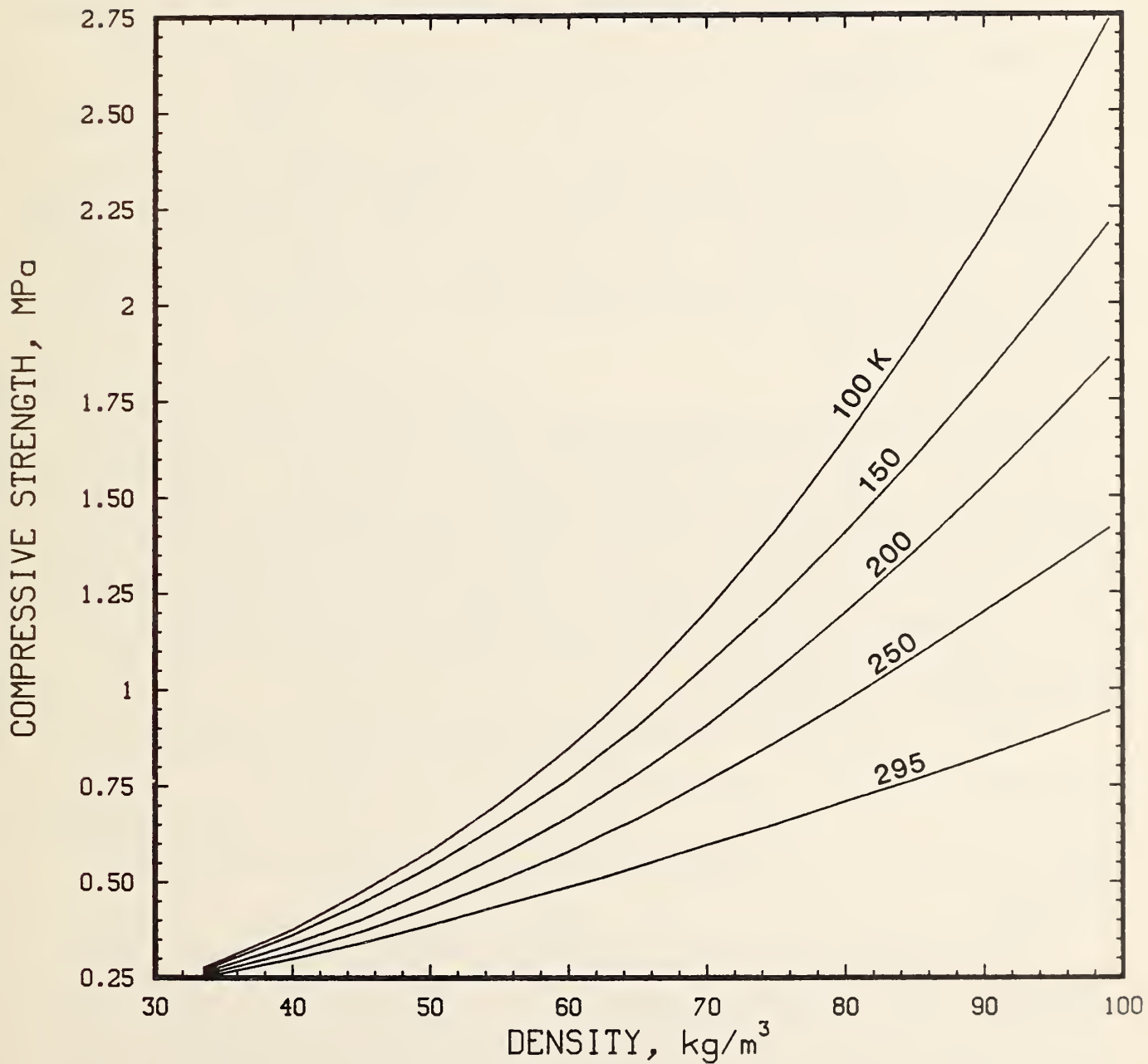
Figure 48. Compressive strength of polyurethane foam as a function of density with temperature as the parameter. The strength obtained here must be modified by a function of (H/W) for a particular material.
