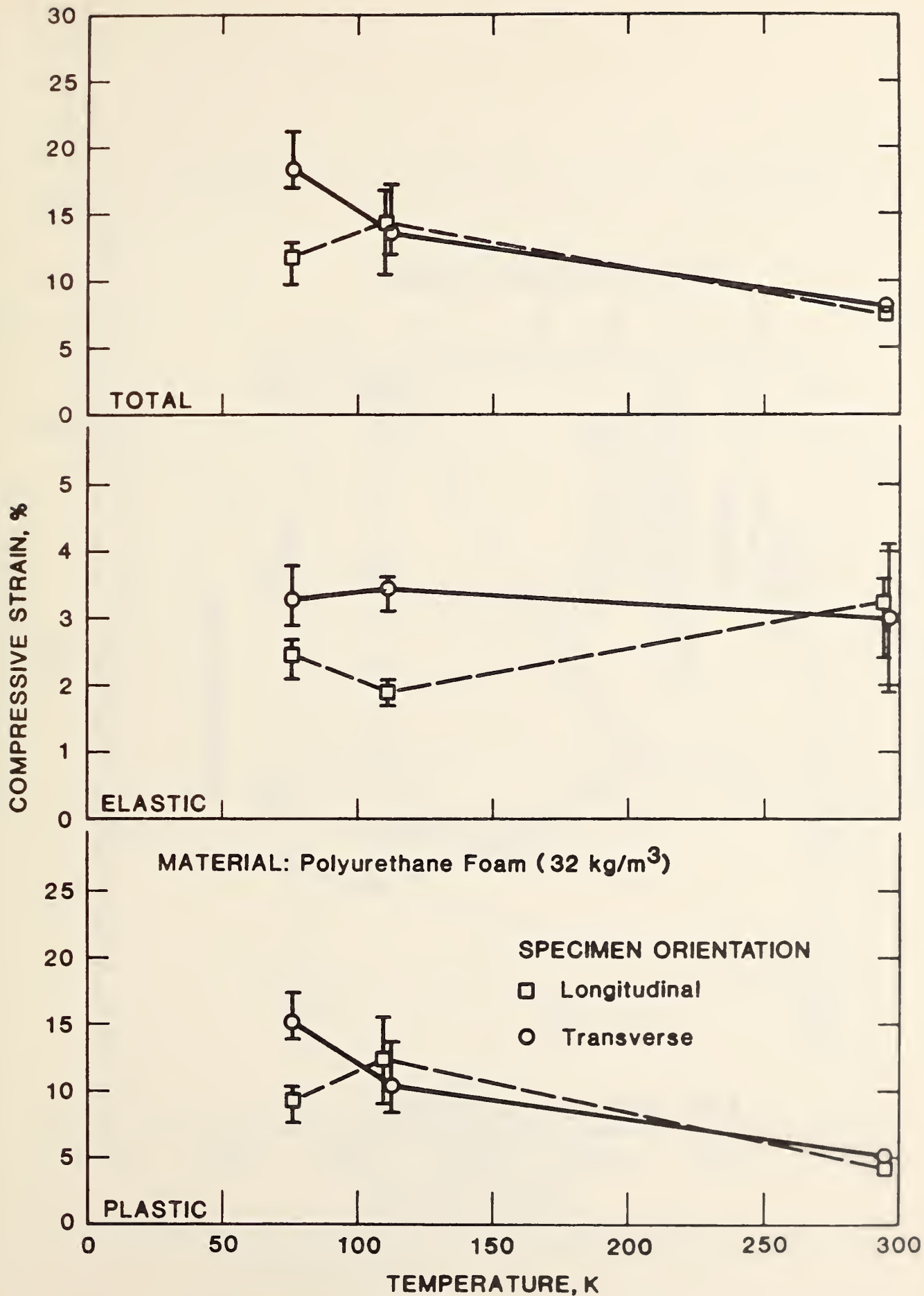
Figure 21. Compressive strain versus temperature for a 32-kg/m 3 polyurethane foam.
