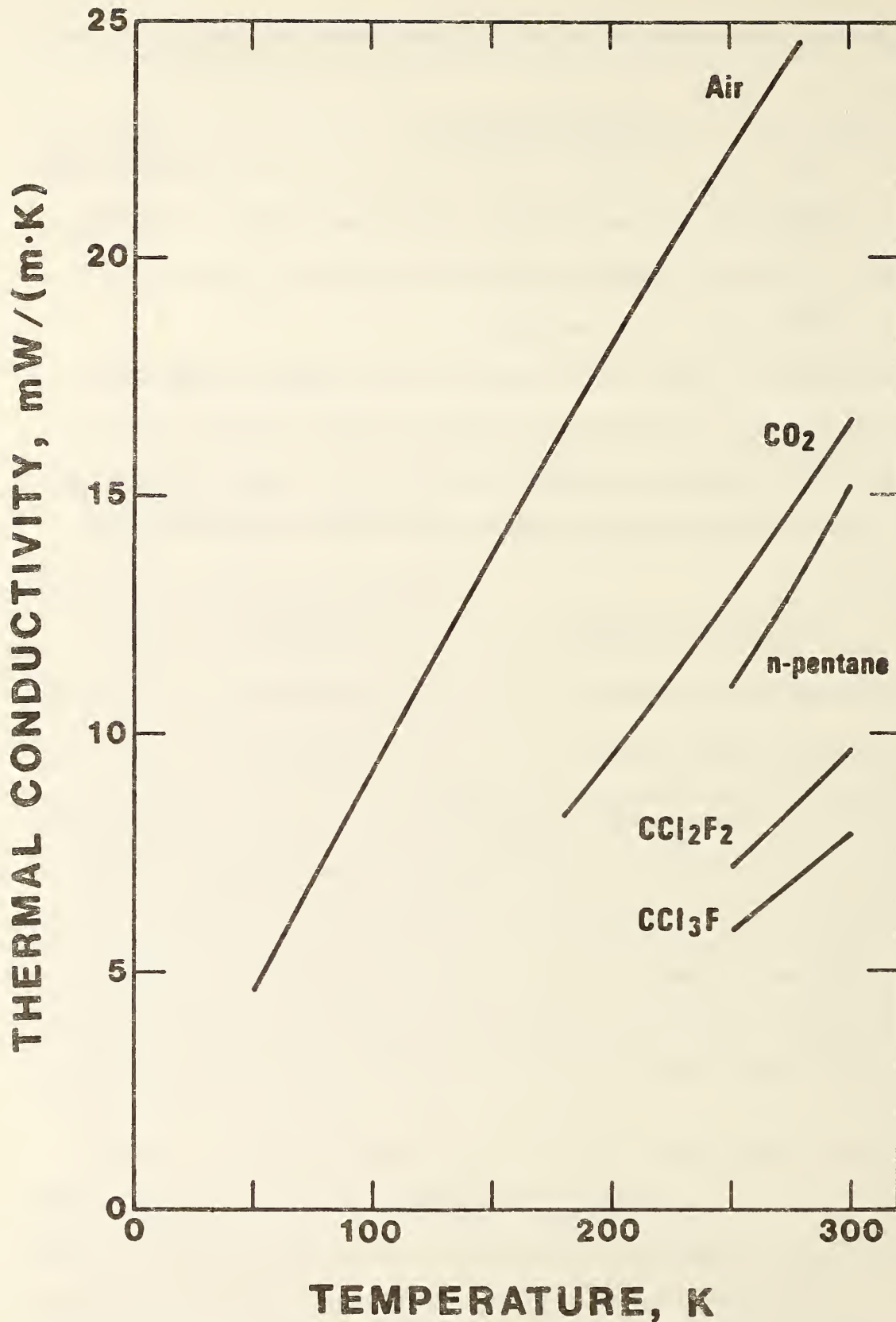
Figure 41. Thermal conductivity as a function of temperature for gases commonly found in polyurethane foams (Touloukian, Liley, and Saxena, 1970).
