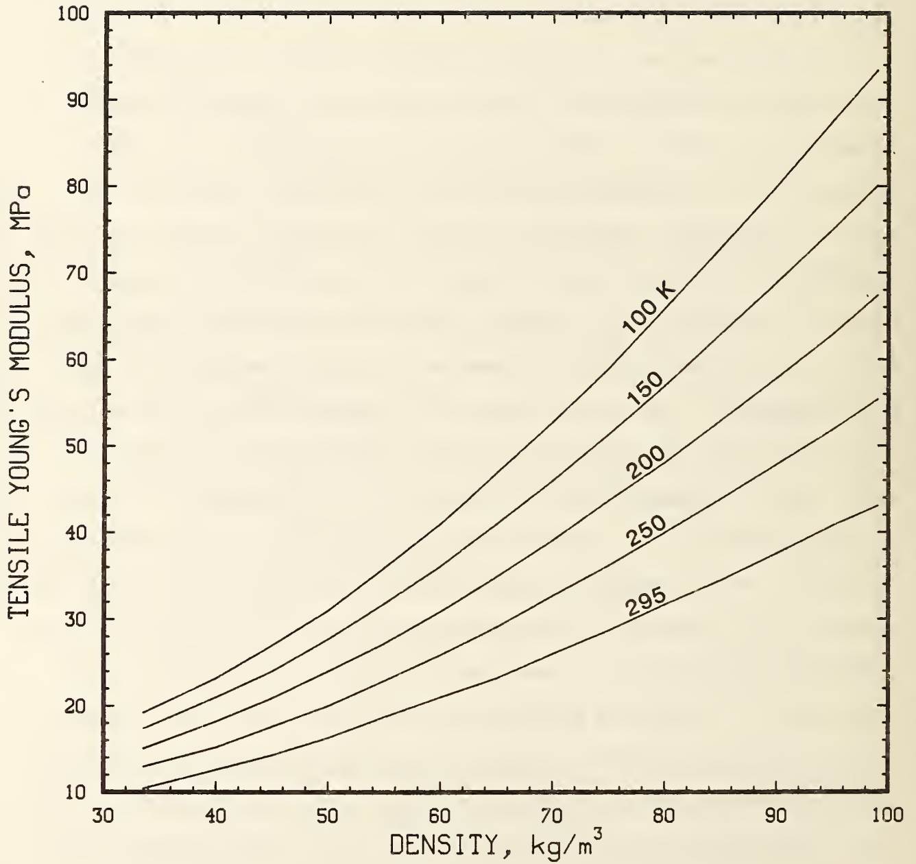
Figure 45. Young's modulus of polyurethane foam in tension as a function of density with temperature as the parameter. The modulus obtained here must be modified by a function of (H/W) for a specific material.
