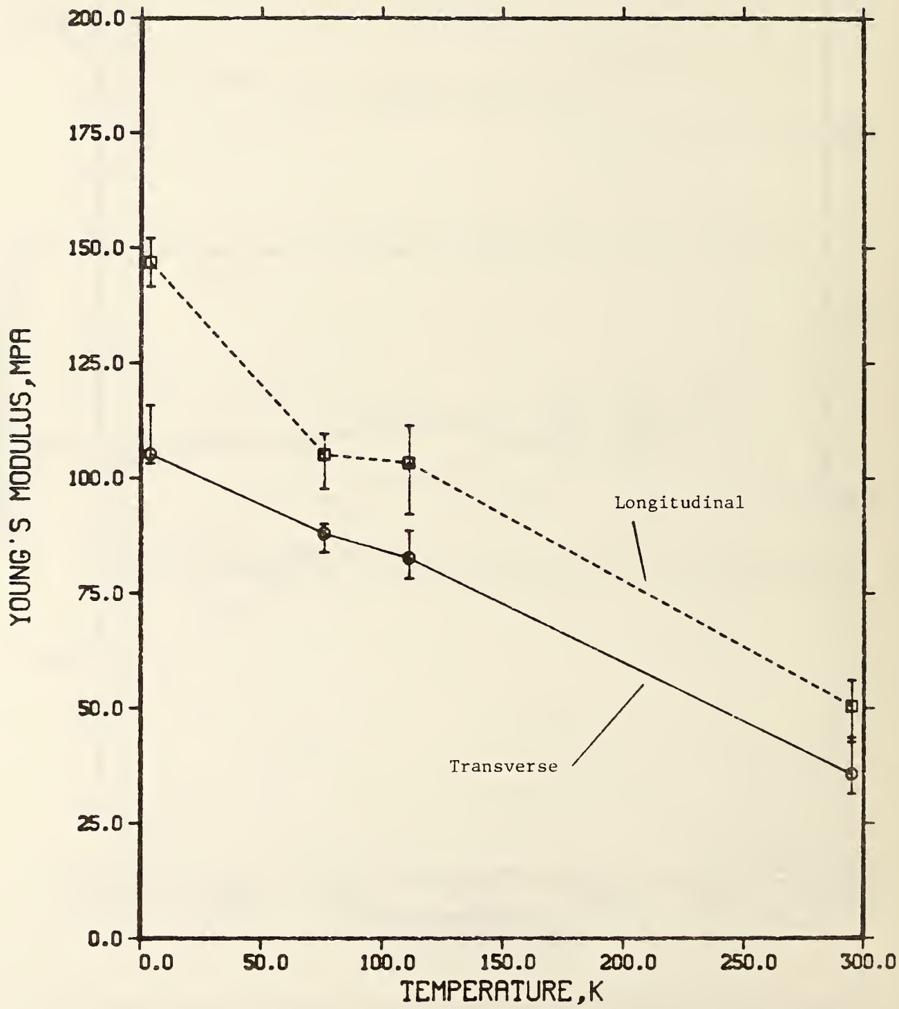
Figure 30. Tensile Young's modulus versus temperature for a 96-kg/m 3 polyurethane foam.
