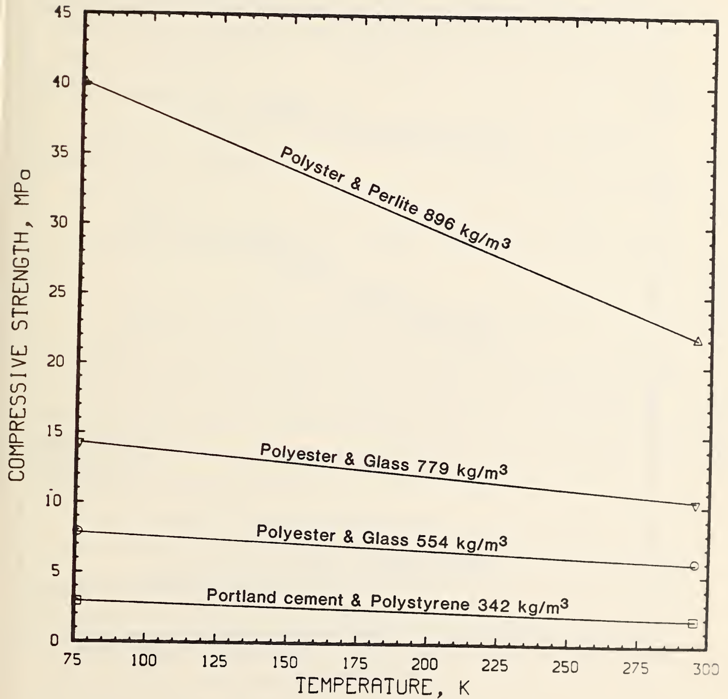
Figure 54. Average compressive strength of several insulating concretes as a function of temperature (determined at NBS).
