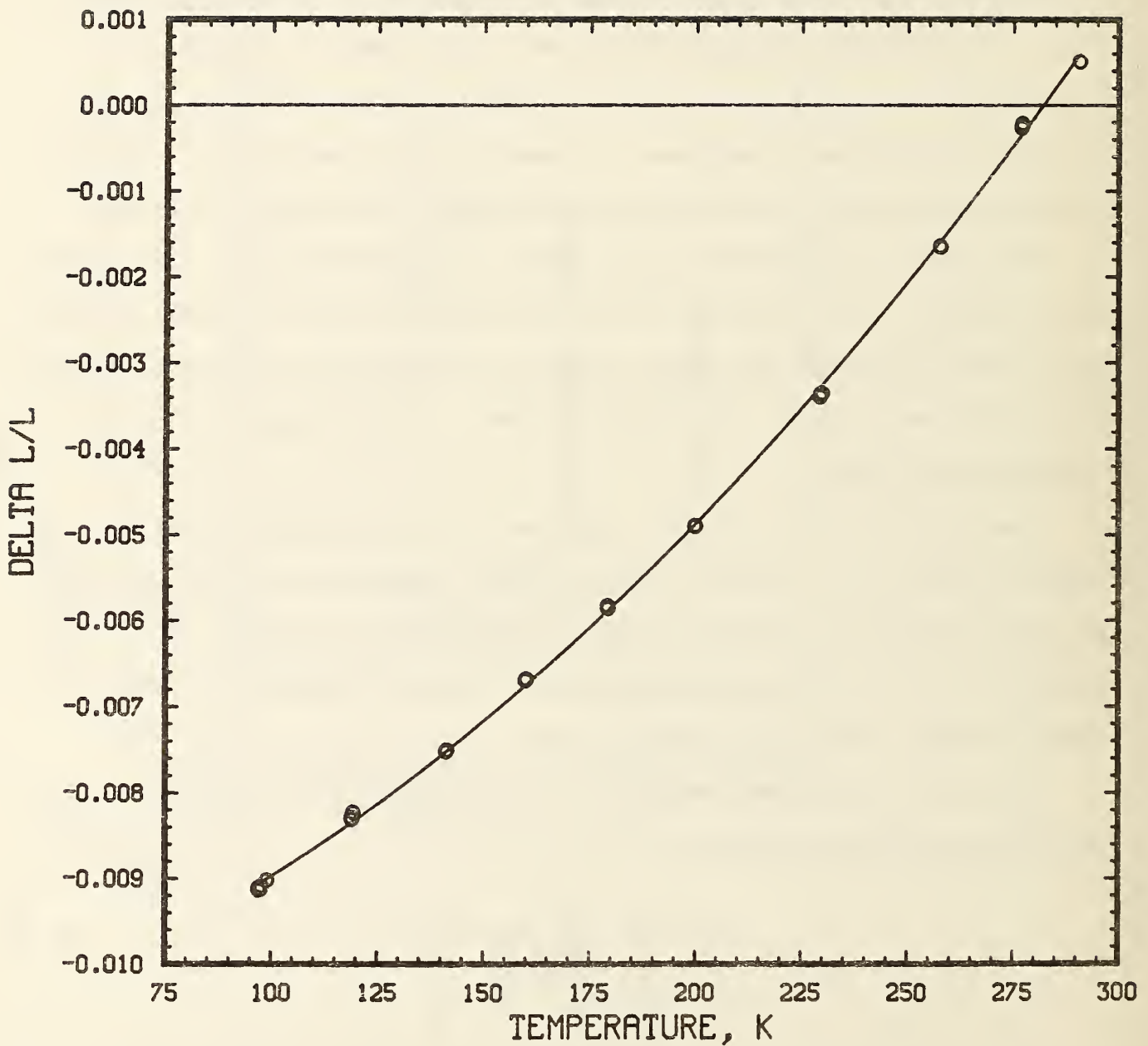
Figure 10. Thermal expansion of a 32-kg/m 3 polyurethane foam specimen. Experimental data are represented by discrete points and the solid line represents a three-term polynomial fit to these data. The reference temperature is 281.997 K.
