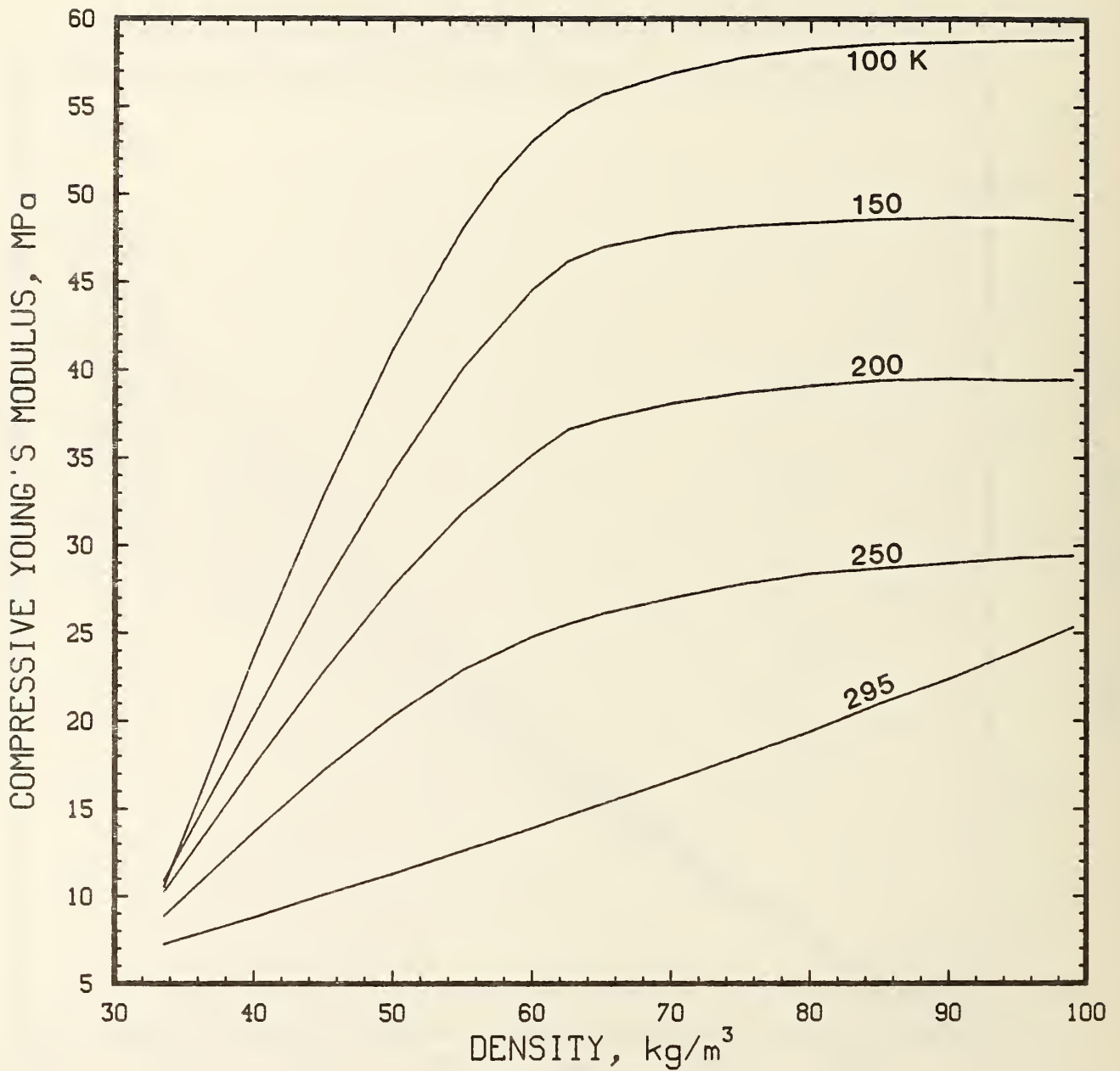
Figure 47. Young's modulus of polyurethane foam in compression as a function of density with temperature as the parameter. The modulus obtained here must be modified by a function of (H/W) for a specific material.
