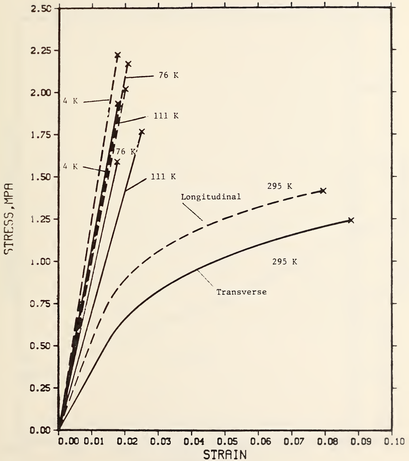
Figure 33. Tensile stress versus strain for a 96-kg/m 3 polyurethane foam.
