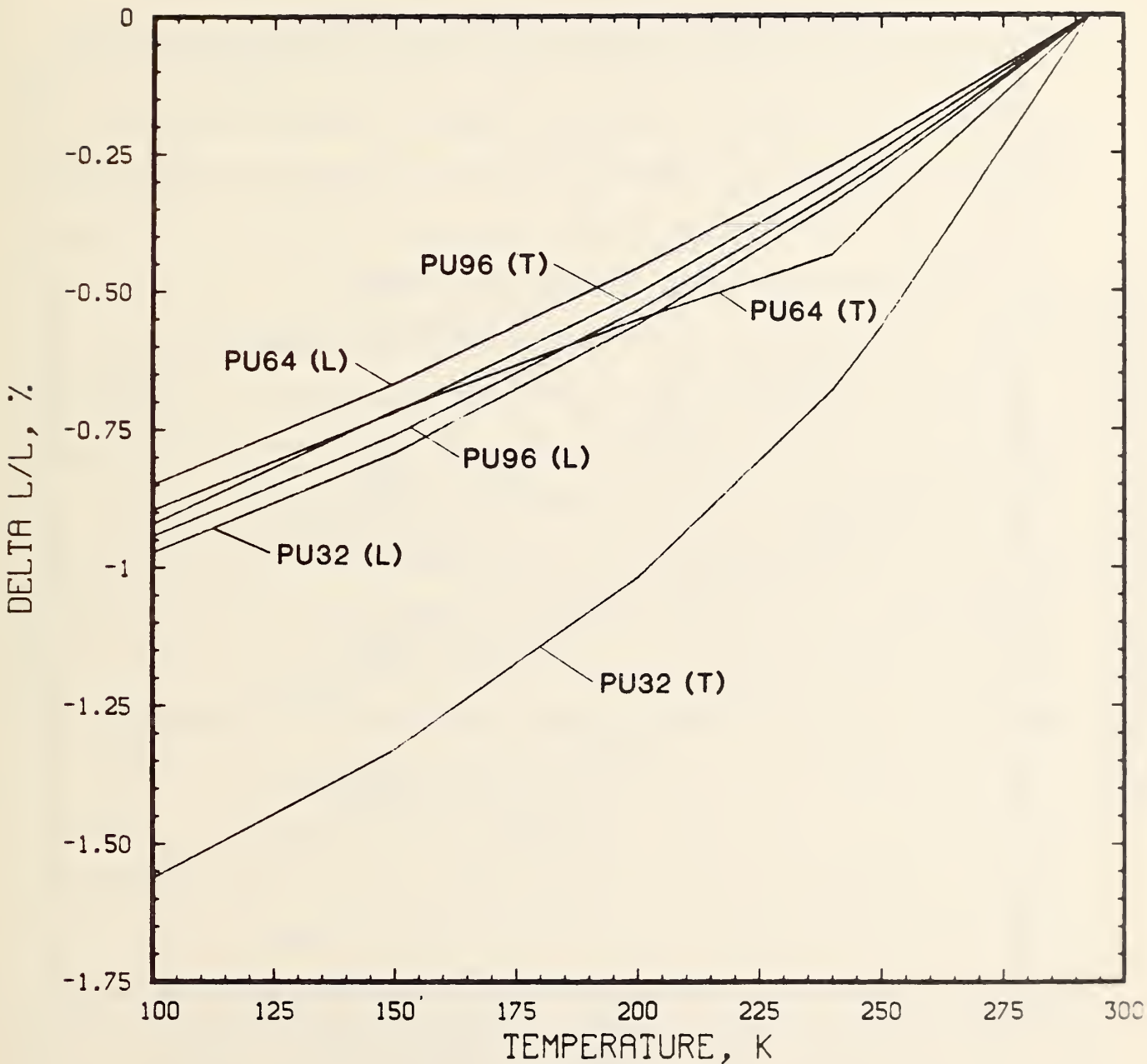
Figure 43. Longitudinal (experimental) and transverse (calculated) thermal contraction of PU32, PU64, and PU96.
