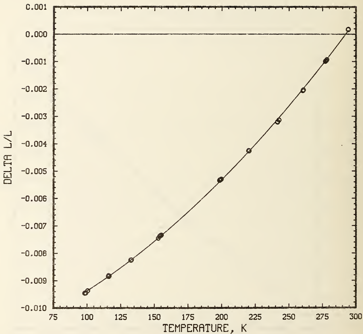
Figure 12. Thermal expansion of a 96-kg/m 3 polyurethane foam specimen. Experimental data are represented by discrete points and the solid line represents a three-term polynomial fit to these data. The reference temperature is 292.227 K.
