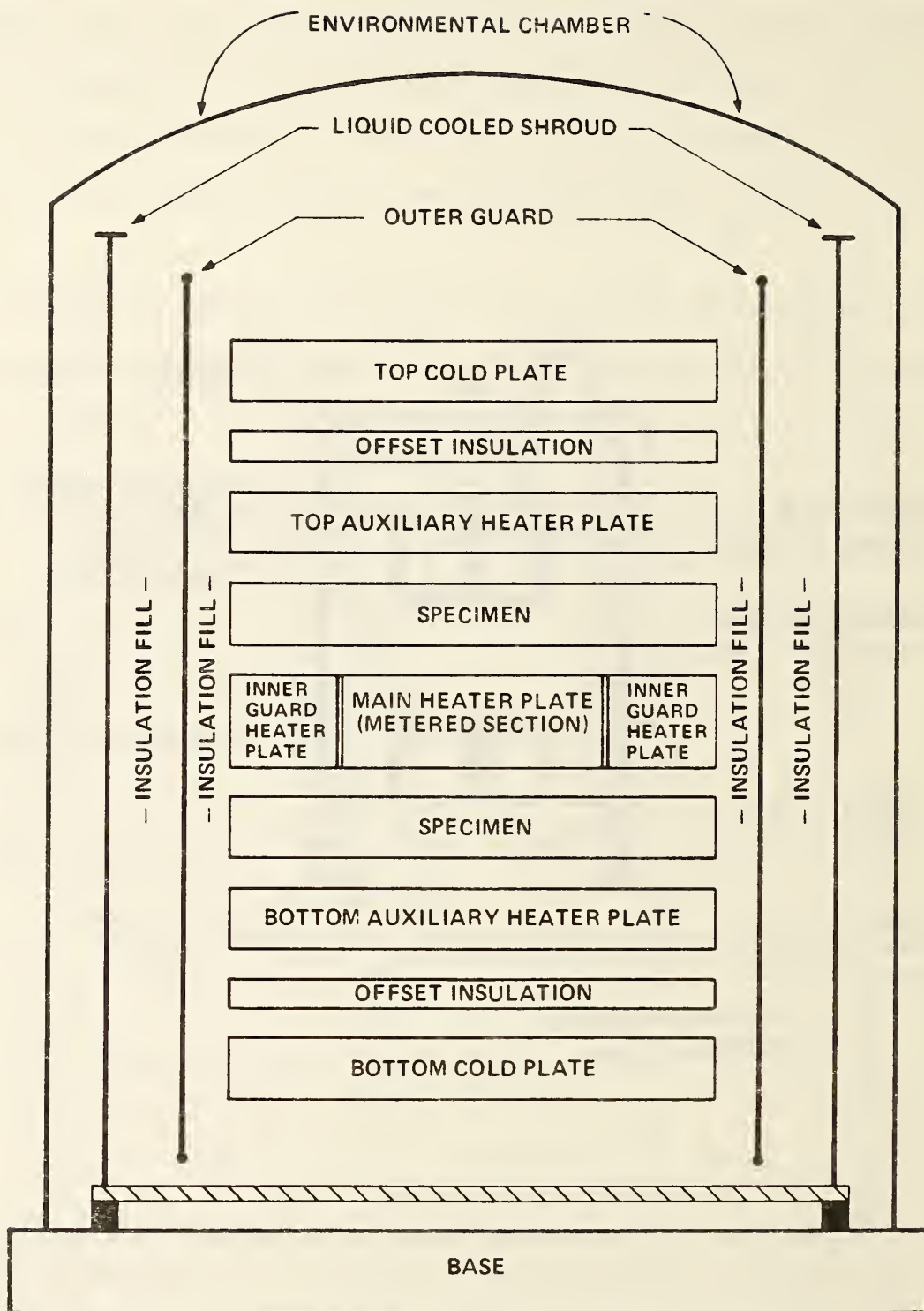
Figure 7. Schematic of guarded-hot-plate specimen configuration and environmental chamber
