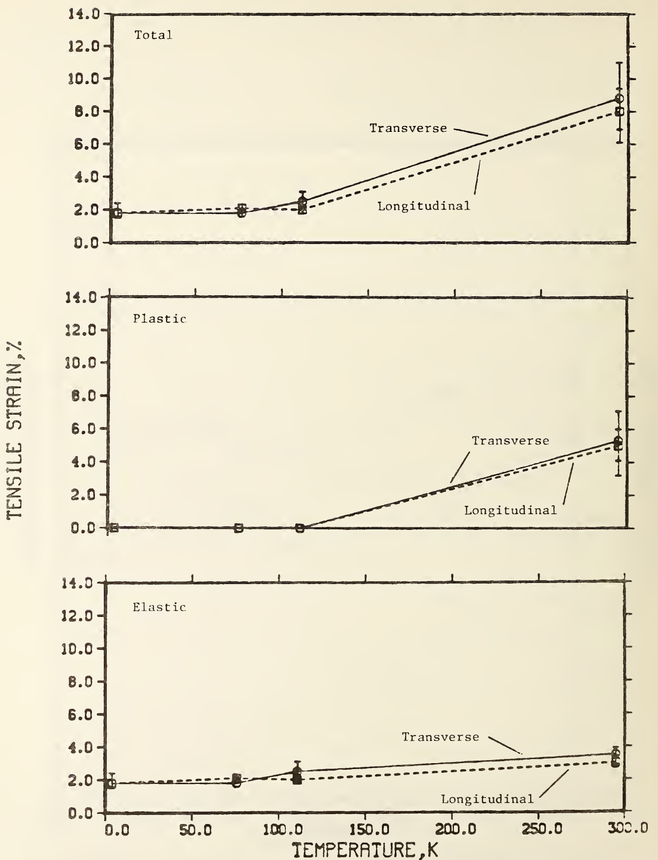
Figure 32. Tensile strain versus temperature for a 96-kg/m 3 polyurethane foam.
