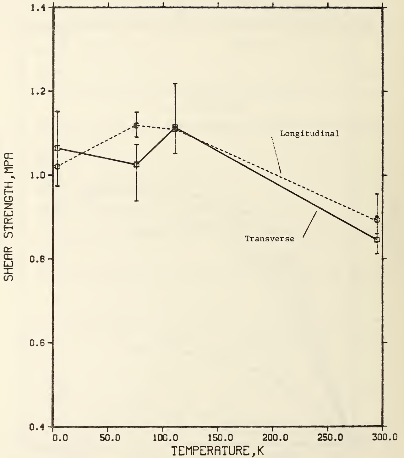
Figure 40. Shear strength versus temperature for a 96-kg/m 3 polyurethane foam.
