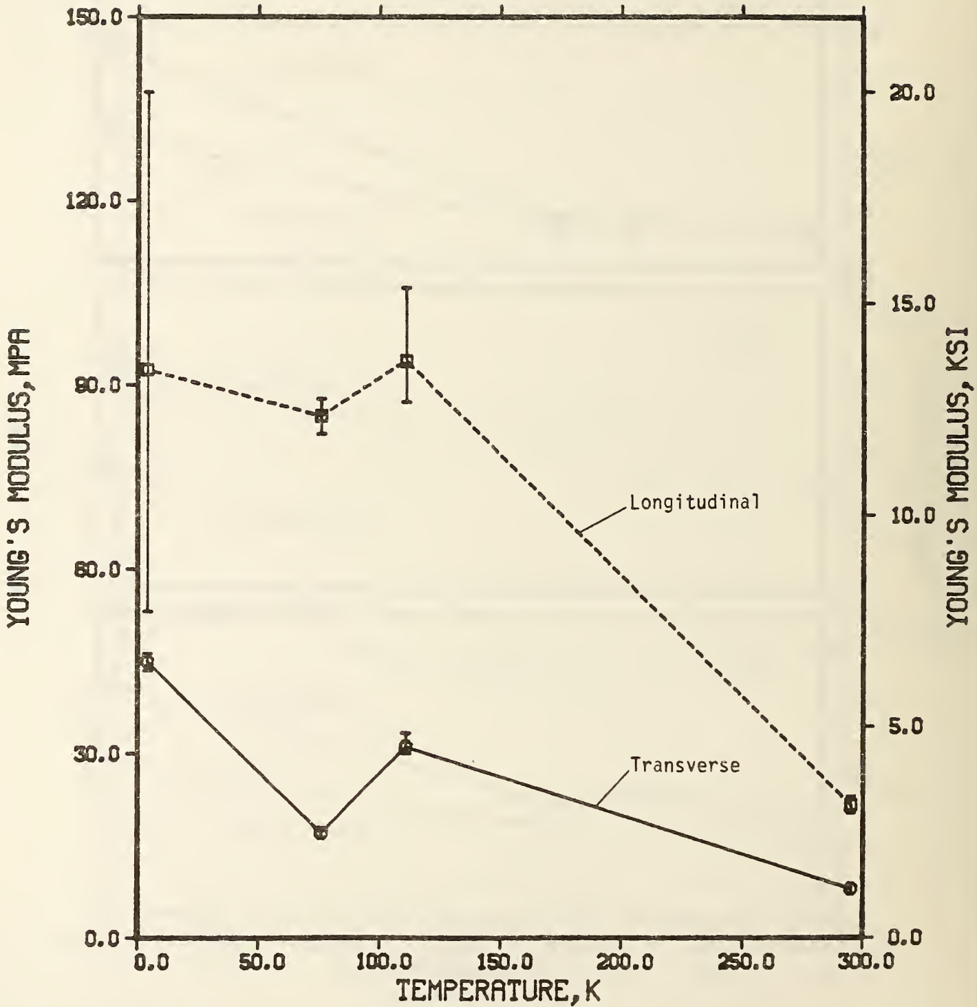
Figure 26. Compressive Young's modulus versus temperature for a 64-kg/m 3 polyurethane foam.
