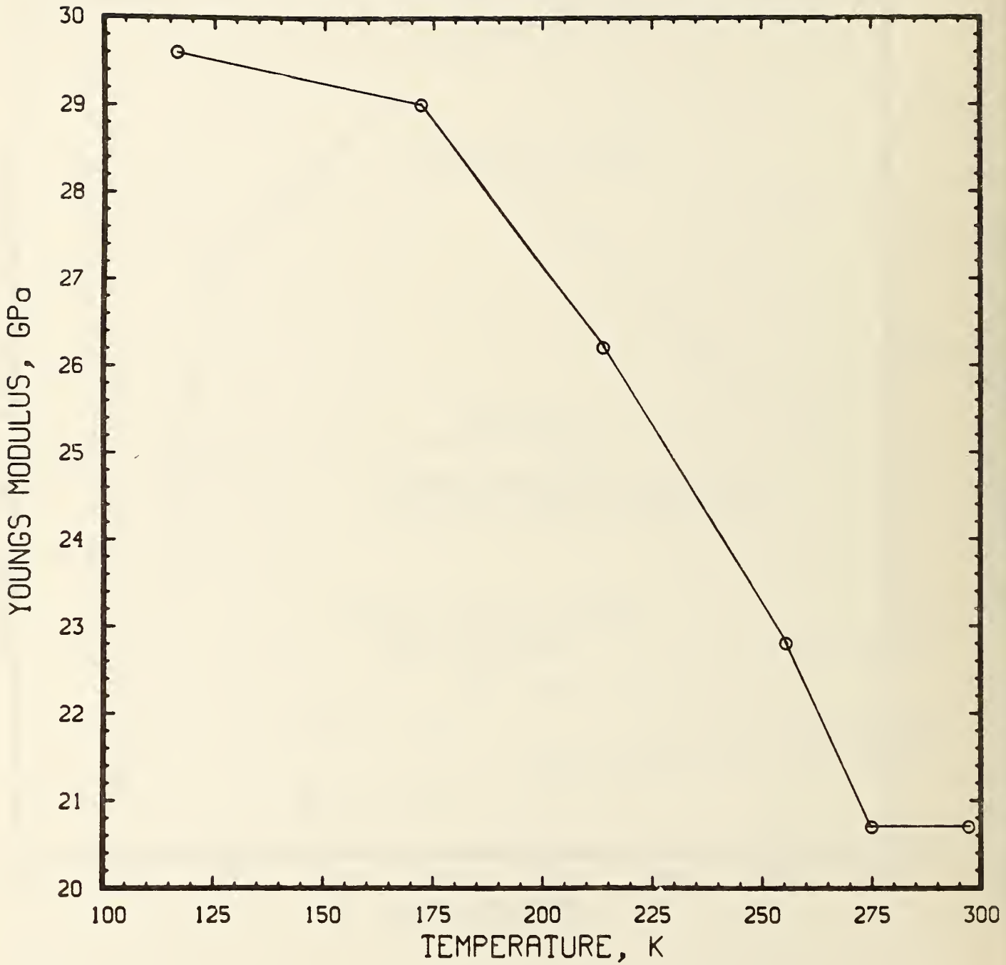
Figure 51. Compressive Young's modulus as a function of temperature for an expanded shale concrete of density 1554 \text{ kg/m}^3 (Monfore and Lentz, 1962).
