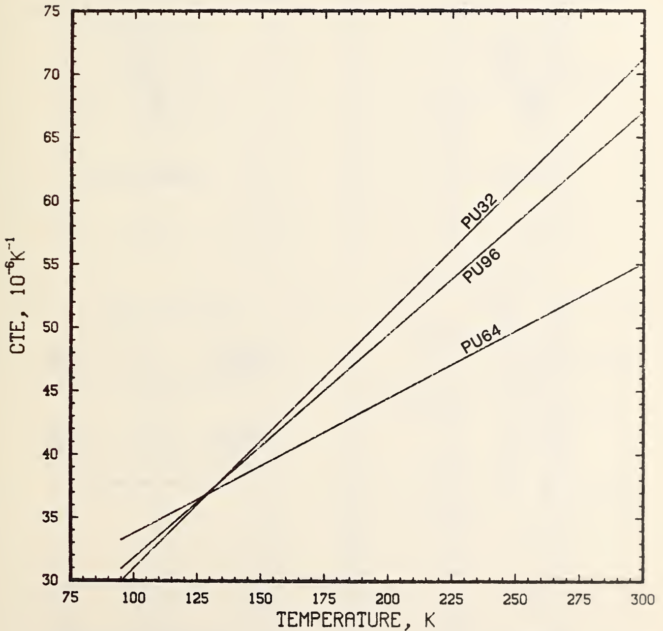
Figure 14. Coefficient of thermal expansion relationships resulting from temperature derivatives of three-term polynomial fits to thermal expansion data of 32-, 64-, and 96-kg/m 3 polyurethane foam specimens.
