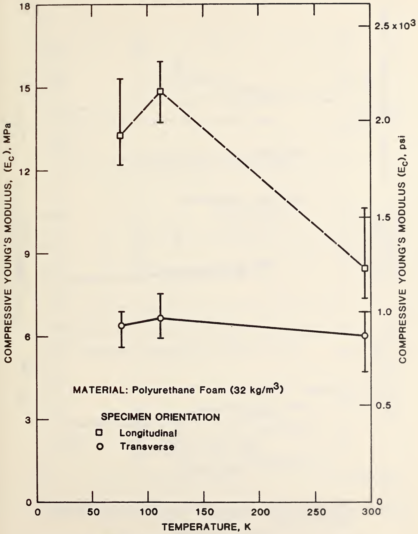
Figure 19. Compressive Young's modulus versus temperature for a 32-kg/m 3 polyurethane foam.
