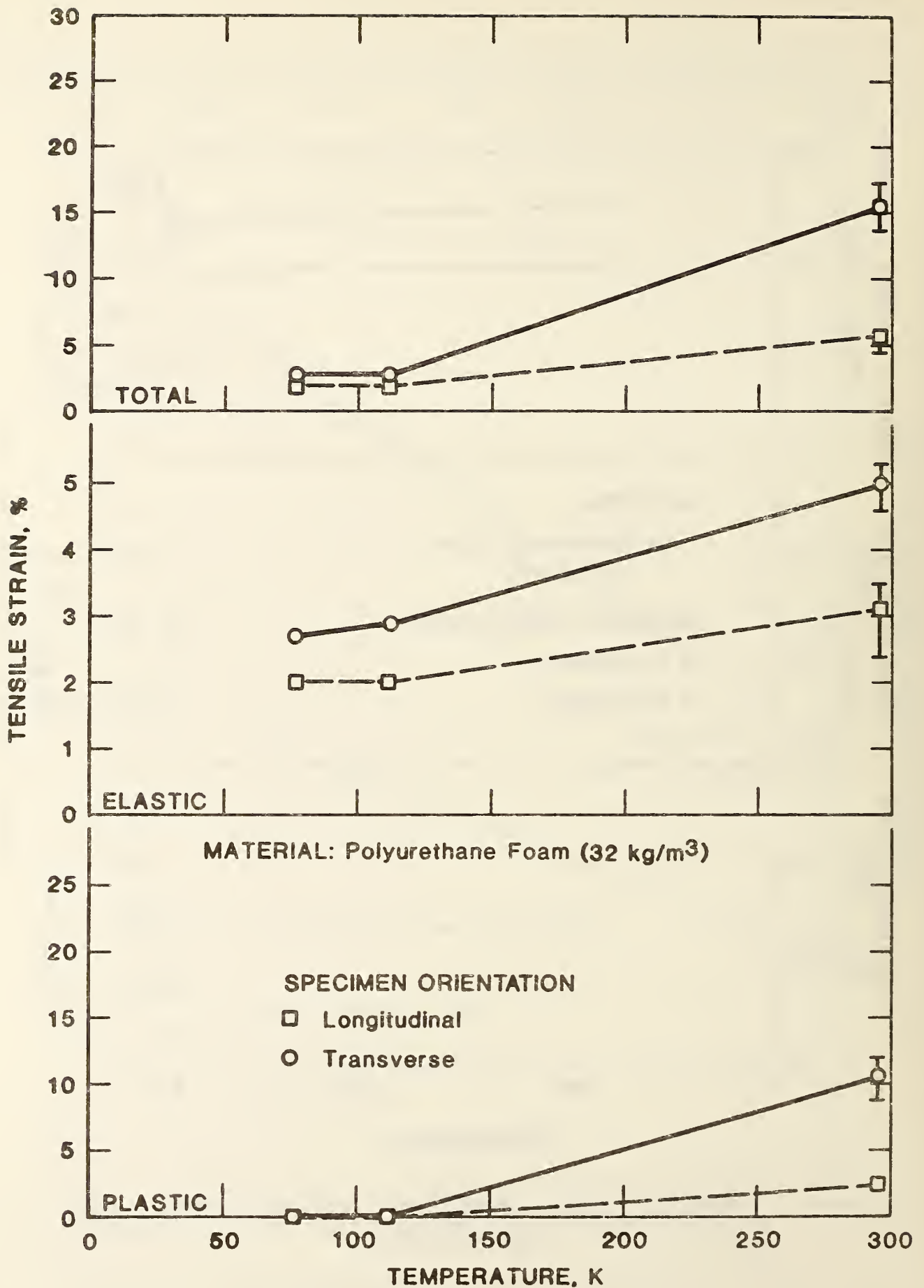
Figure 18. Tensile strain versus temperature for a 32-kg/m 3 polyurethane foam.
