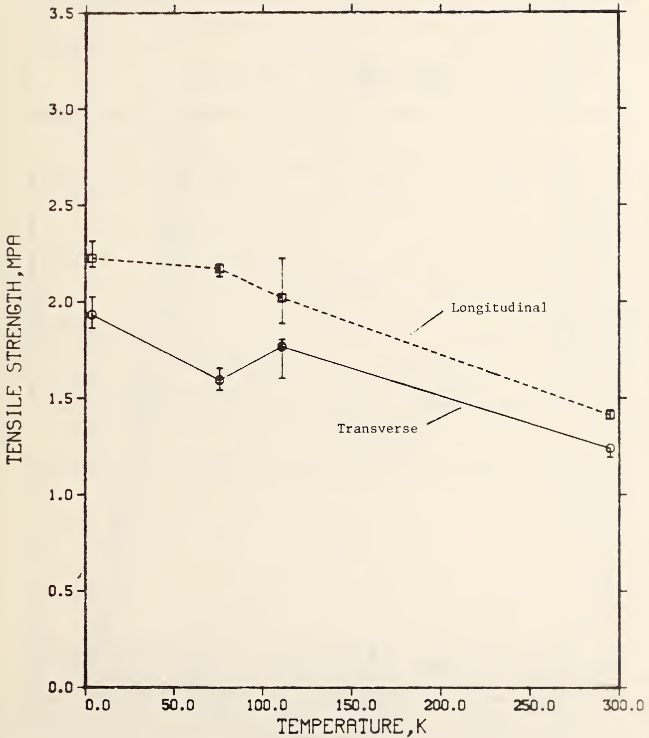
Figure 31. Ultimate tensile strength versus temperature for a 96-kg/m 3 polyurethane foam.
