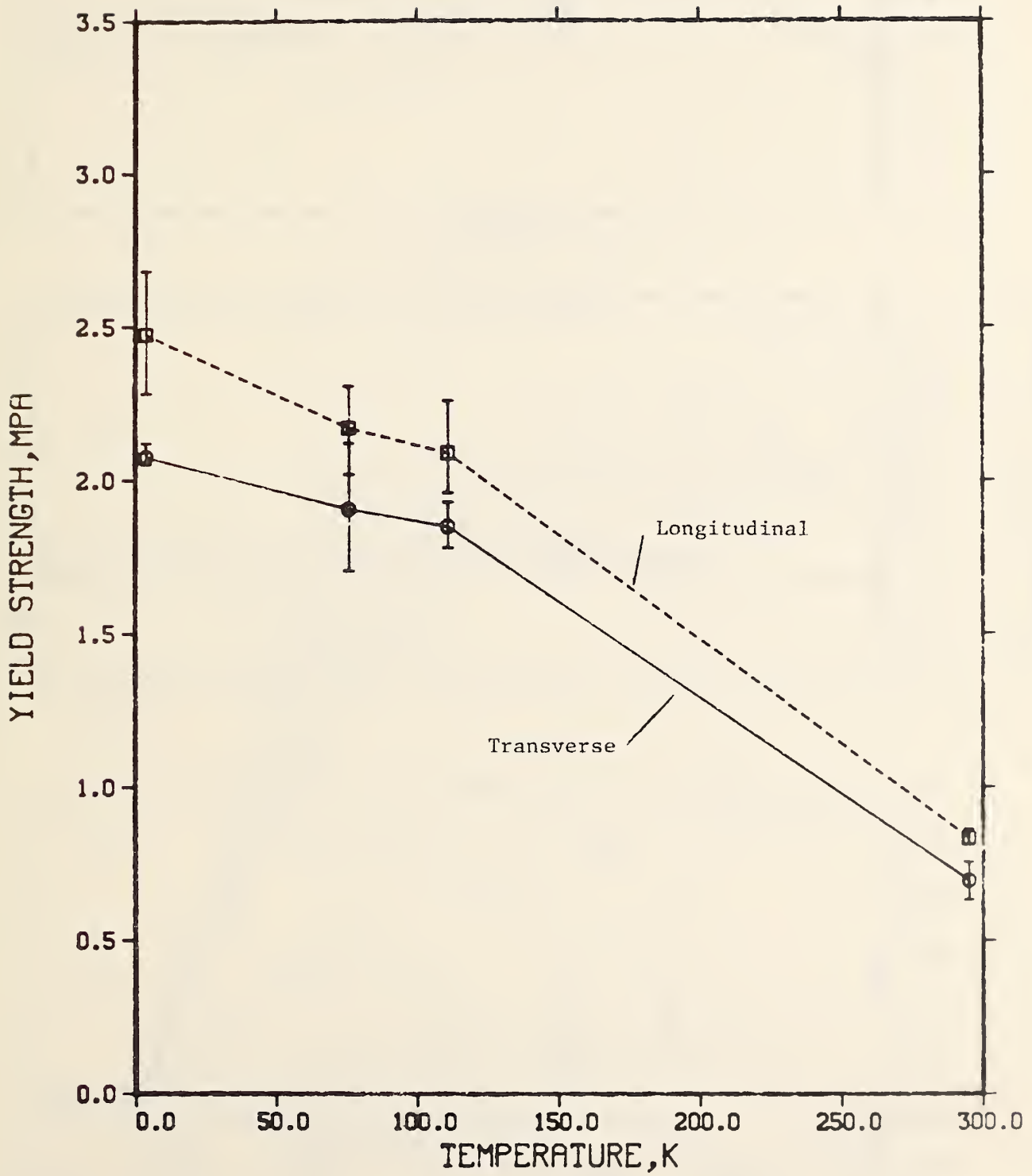
Figure 37. Compressive yield strength versus temperature for a 96-kg/m 3 polyurethane foam.
