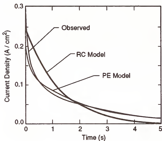
Figure 3. Observed discharge performance versus porous electrode distributed model (PE) and simple resistive model (RC) for test device illustrated in Fig. 5 and for 600 \text{ mg/cm}^3 carbon aerogel, R/C = 200 , from 0.1 to 0.0 V.
