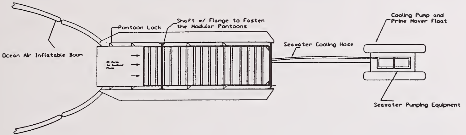
Modular In-Situ Burning Barge Emergency Transport by Plane, Truck or Water.
