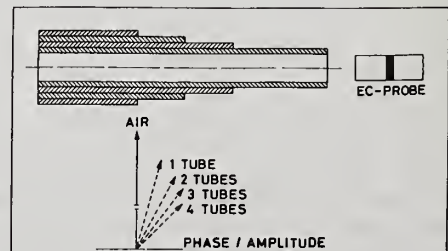
Figure 1. Phase relationships.
