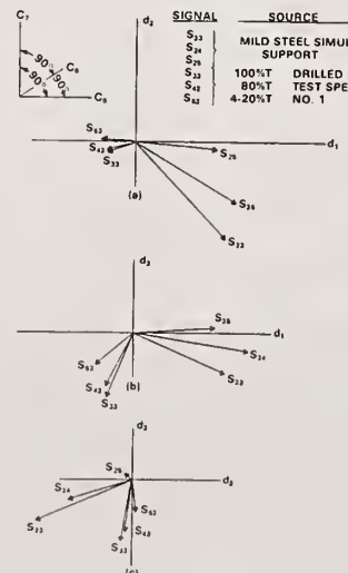
Figure 8. Three 2-space views of signals in 3-space.
