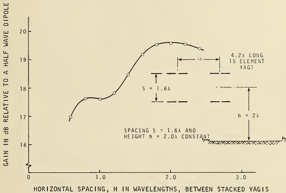
FIG. 12 GAIN OF AN ARRAY OF TWO SETS OF STACKED YAGIS SPACED 1.6\lambda AS A FUNCTION OF HORIZONTAL DISTANCE BETWEEN THEM
