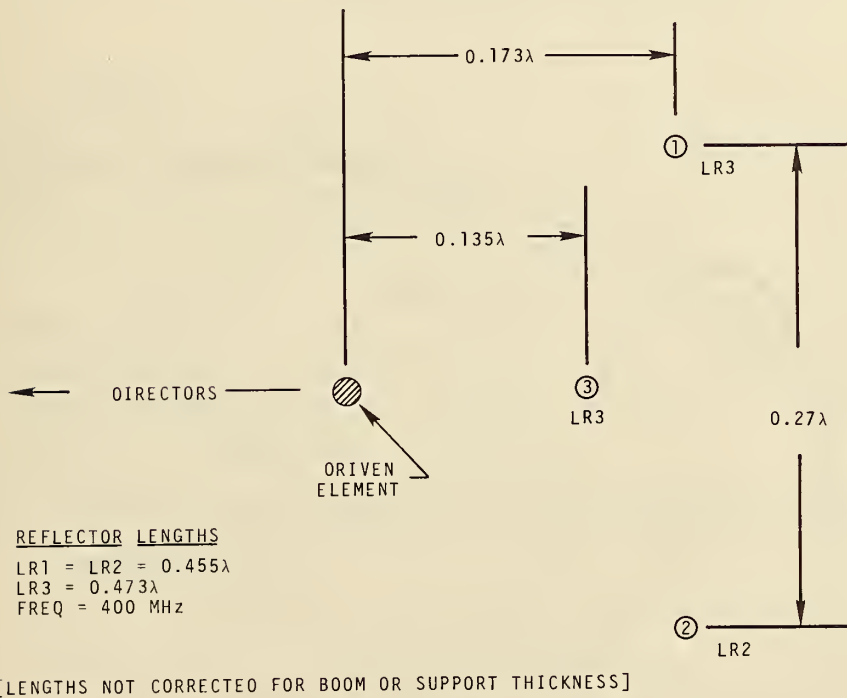
FIG. 2 ARRANGEMENT OF THREE REFLECTING ELEMENTS USED WITH THE 4.2λ YAGI
