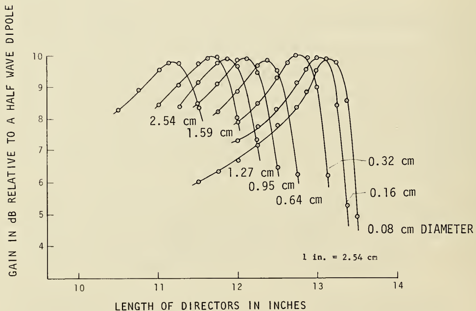
FIG. 8 MEASURED GAIN VS DIRECTOR LENGTH OF A 1.25\lambda YAGI ANTENNA USING THREE DIRECTORS OF DIFFERENT LENGTH AND DIAMETER SPACED 0.35\lambda
