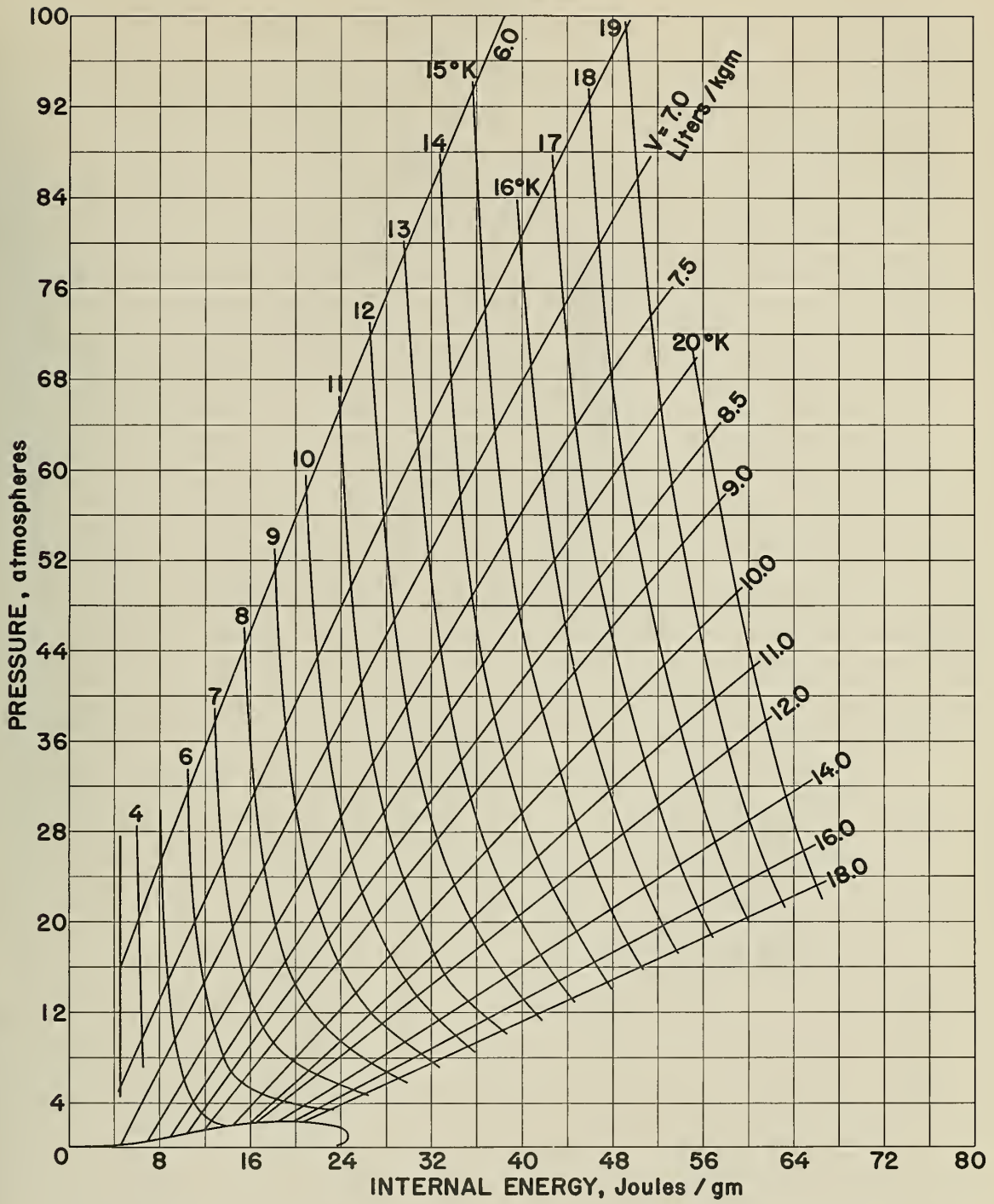
Figure 12. Pressure-Internal Energy Diagram for Helium 0 - 100 Atmospheres
