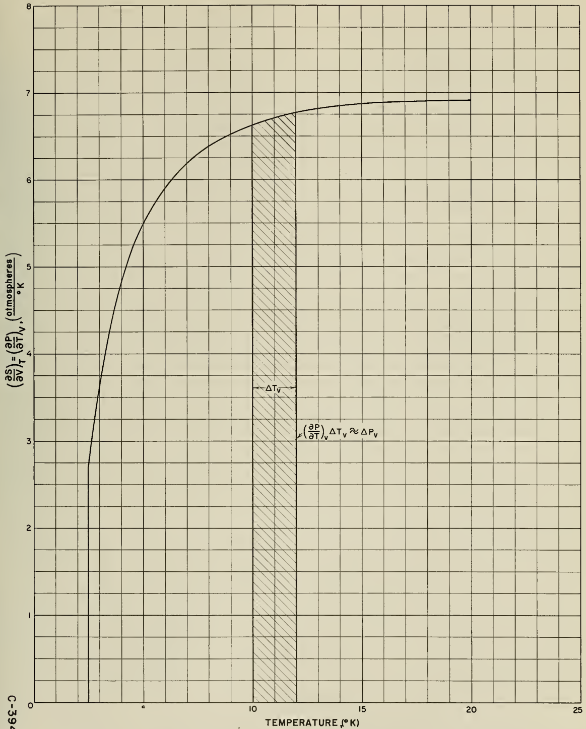
Figure 8. Slopes of Isotherms of Figure 7 Illustrating the Method Used to Determine Isobars.
