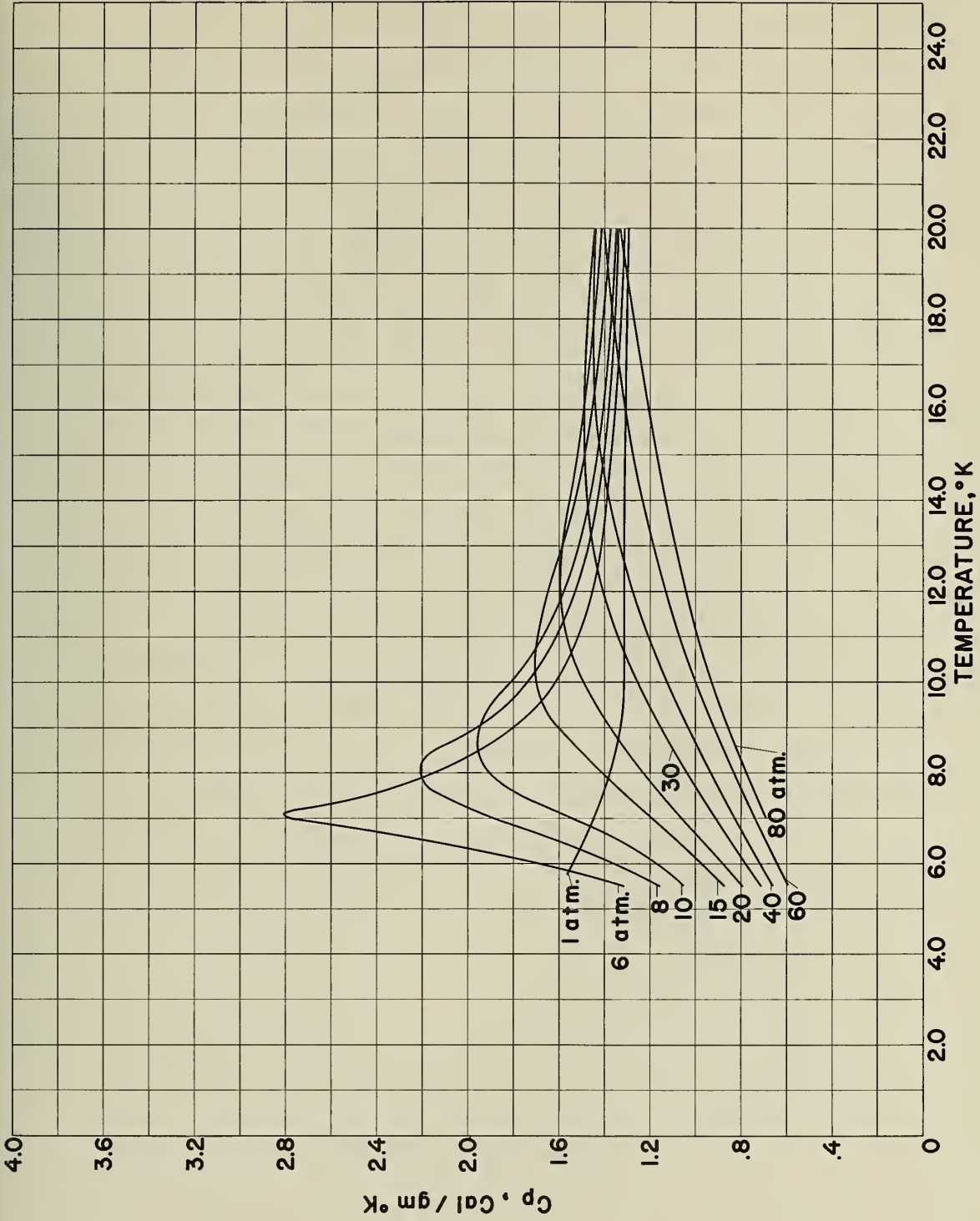
Figure 13. Specific Heat at Constant Pressure of Helium Gas
