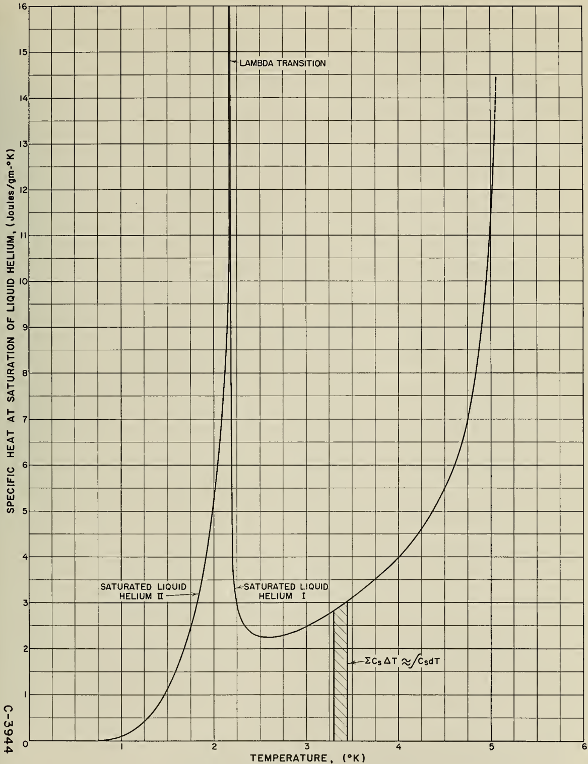
Figure 2. Specific Heat at Saturation of Liquid Helium Illustrating the Method Used to Calculate \int C_{sat} dT Employed to Determine the Absolute Enthalpy of Liquid Helium at The Normal Boiling Point.
