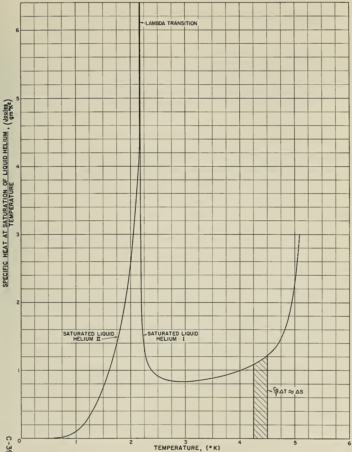
Figure 1. Specific Heat at Saturation of Liquid Helium Illustrating the Method Used to Determine the Absolute Entropy of Liquid Helium at the Normal Boiling Point.
