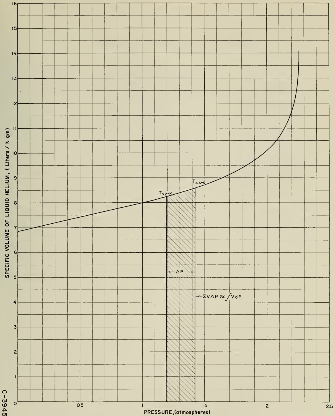
Figure 3. Specific Volume of Saturated Liquid Helium Illustrating the Calculation of \int V dp Used in Determining the Enthalpy at the Normal Boiling Point.
