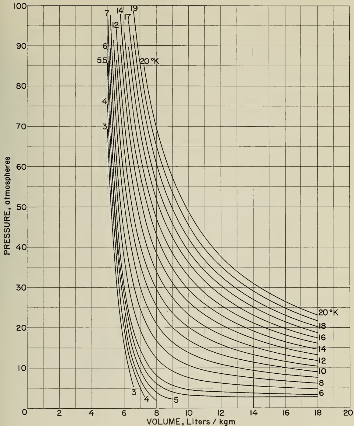
Figure 10. Pressure-Specific Volume Diagram for Helium(Lounasmaa)
