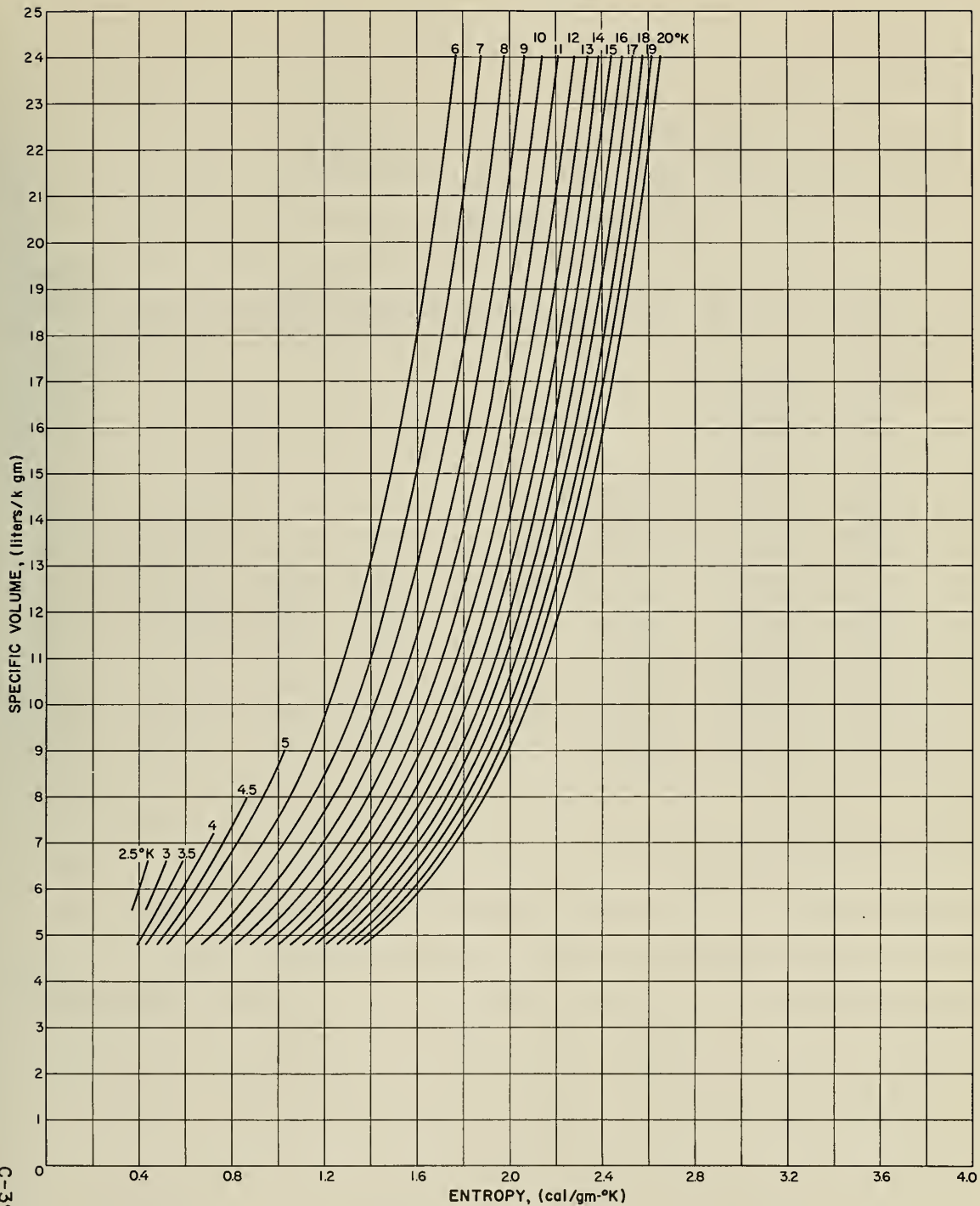
Figure 7. Isotherms of Helium as Functions of Volume and Entropy.
