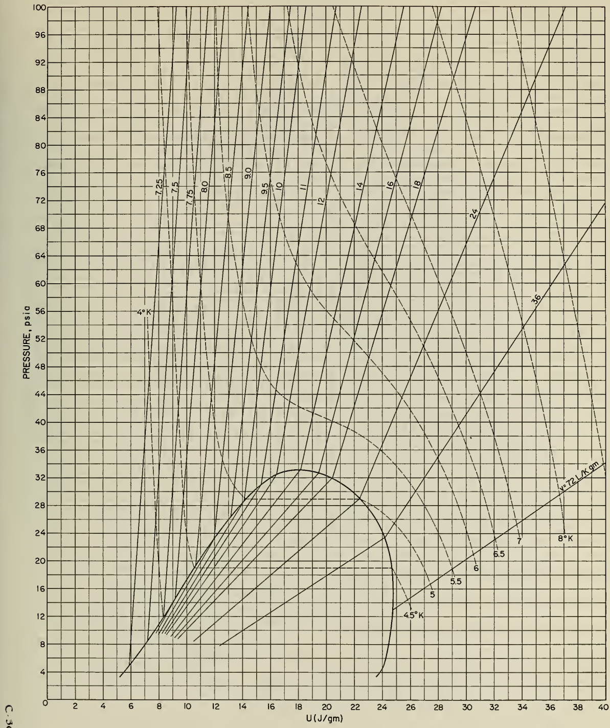
Figure 11. Pressure-Internal Energy Diagram for Helium 0 - 100 psia
