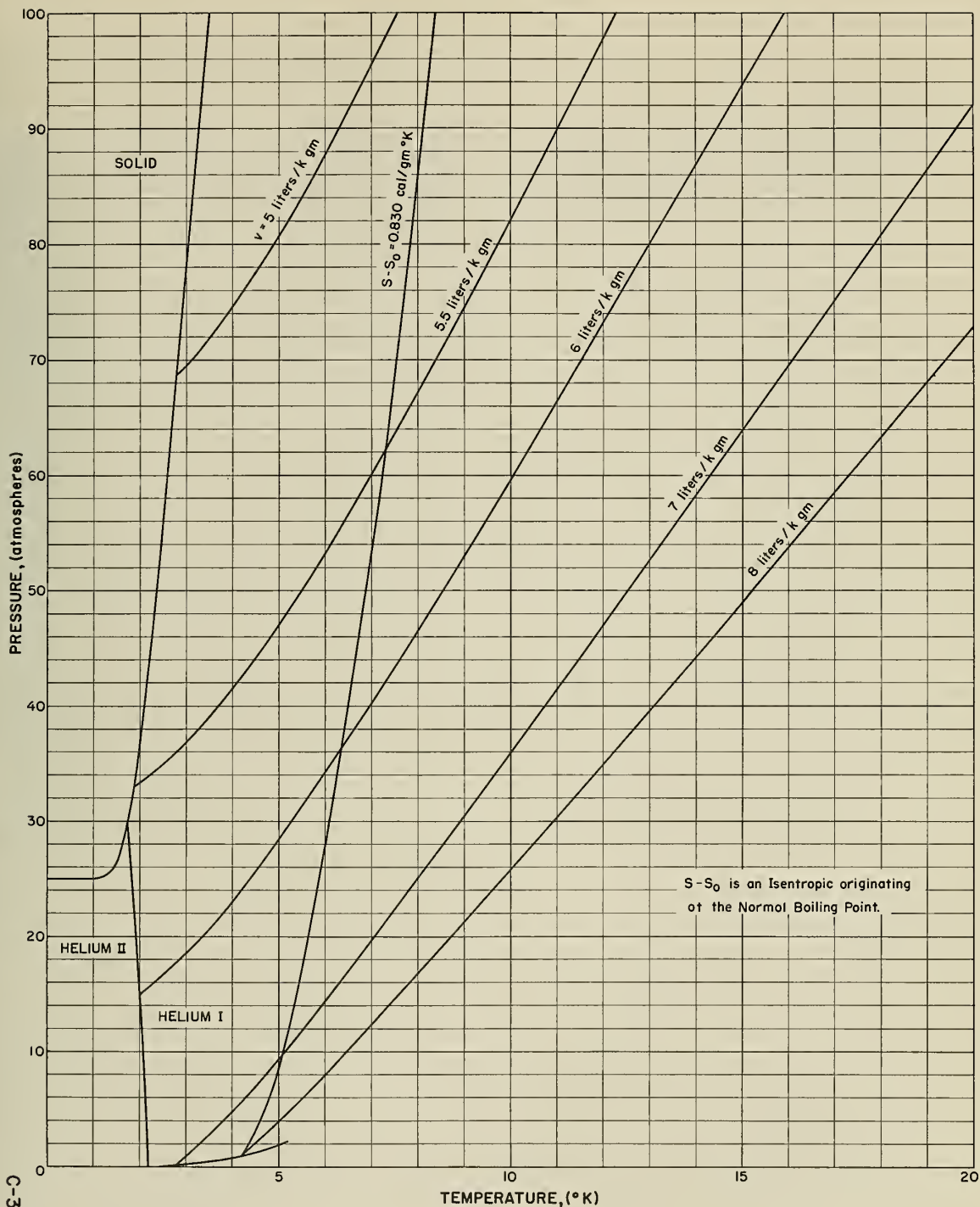
Figure 9. Pressure-Temperature Diagram of Helium Illustrating the Method Used to Determine Enthalpy Values
