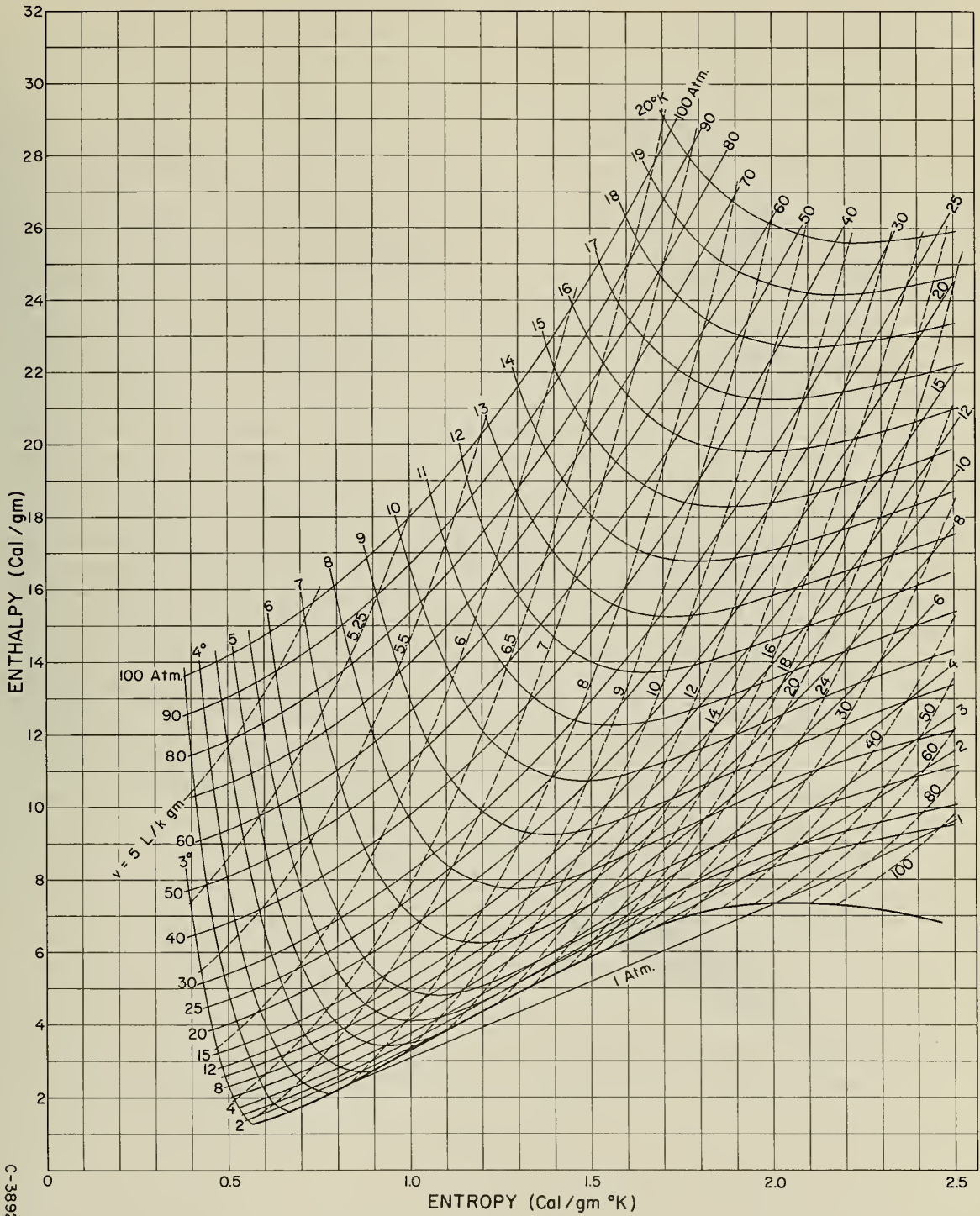
Figure 4. Enthalpy-Entropy Diagram of Helium
