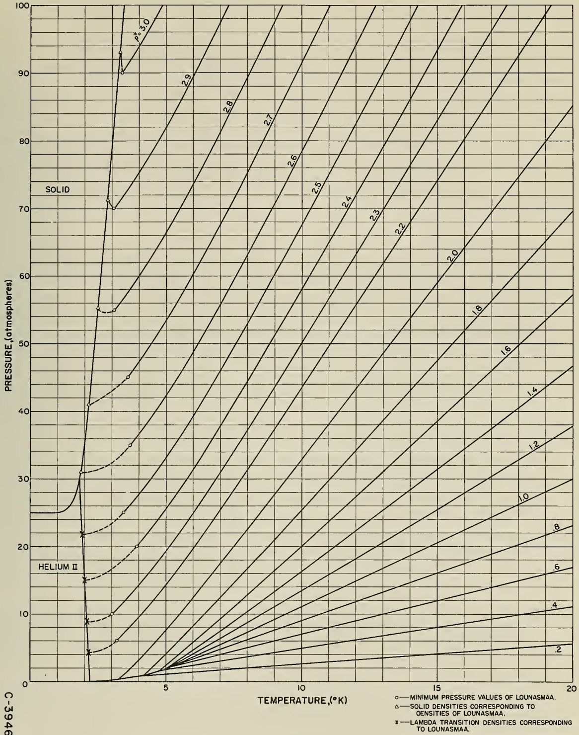
Figure 6. Pressure-Temperature Diagram of Helium
