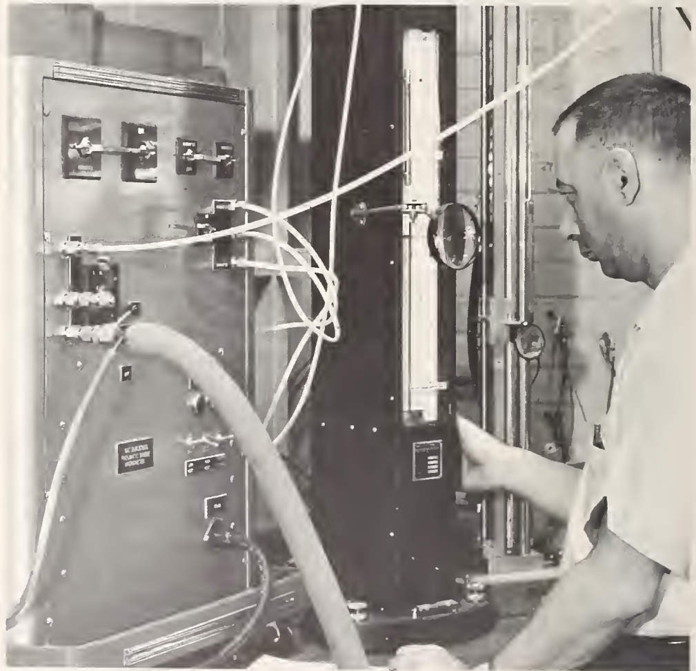
Pneumatic bridge hygrometer developed for use as a secondary or laboratory reference standard for humidity measurements. (See p. 144.)
