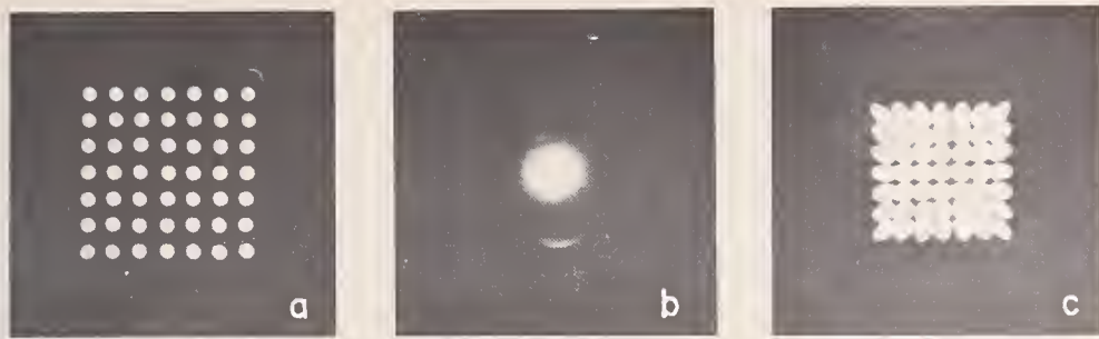
Images, photographed at various focal planes on the lens axis, formed by placing a perforated plate on the front surface of a long focal length lens and illuminating it with collimated light. These "spot diagrams" aid in the determination of the geometrical properties of the lens. (A) taken on the lens side of the position of best focus; (B) taken at the position of best focus; (C) taken beyond the position of best focus. (See p. 30.)
