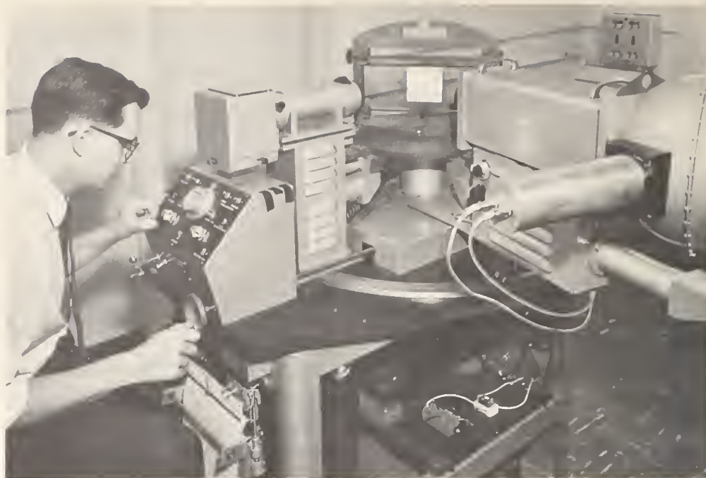
Measurement of reflective properties of materials used for balloon satellites. The measurements will provide a basis for analysis of the effect of radiation pressure on such satellites. (See p. 34.)
