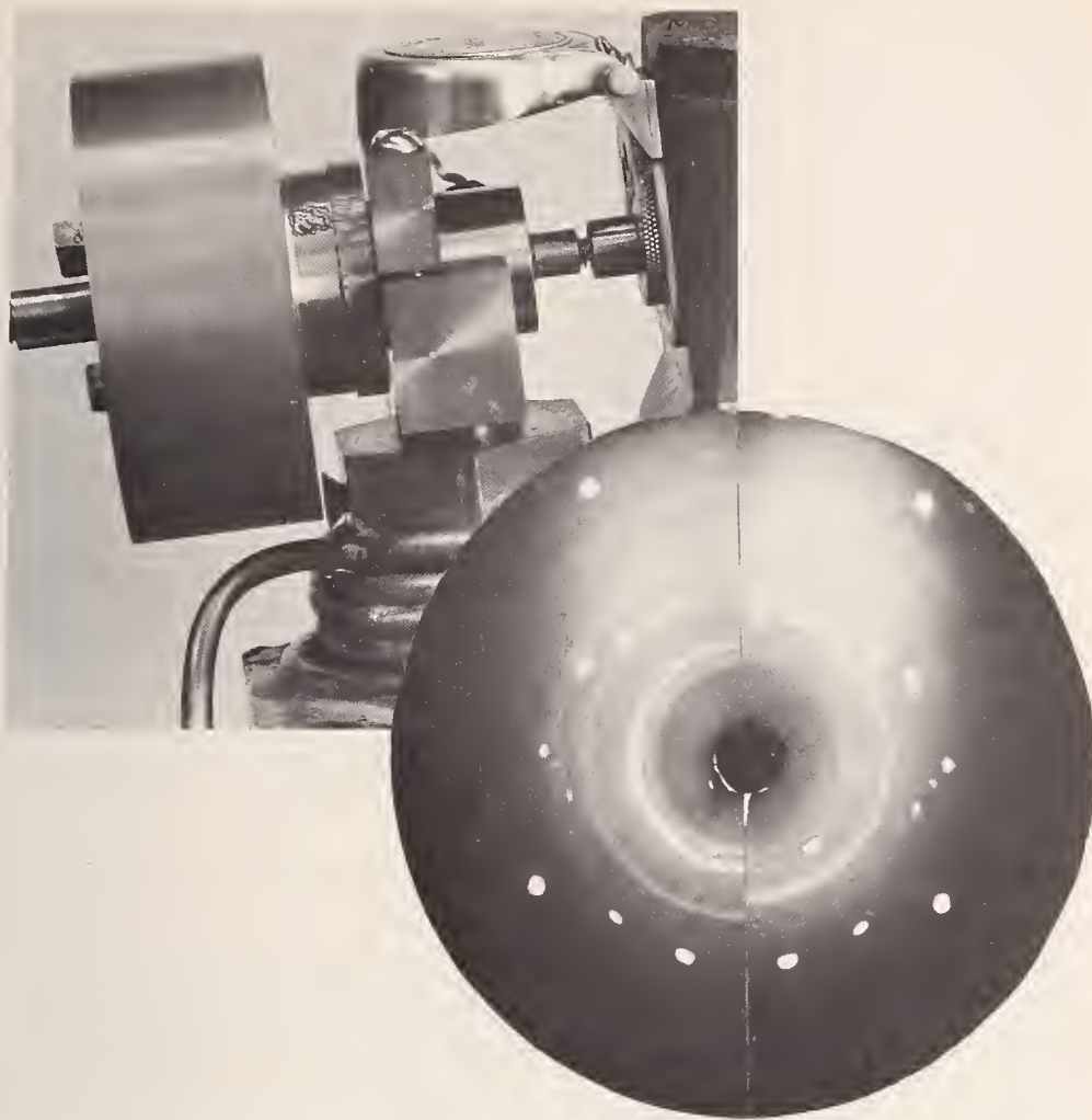
Left: X-ray diffraction camera which incorporates an opposed diamond-anvil pressure cell. Right: Matched X-ray powder diffraction patterns of potassium iodide showing high- and low-pressure forms. Left half represents the normal face-centered cubic structure at 1 bar. Right half, at 20 kilobars, shows a simple cubic structure. The pattern of the salt is shown by the rings and arcs. The spots are due to diffraction from the diamonds. (See p. 106.)
