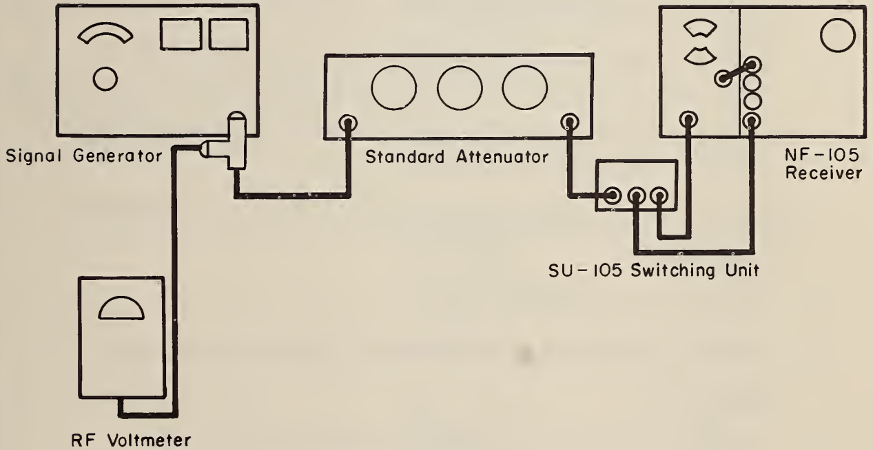
Figure 4.1. Overall Linearity Calibration System Cabling Diagram.
