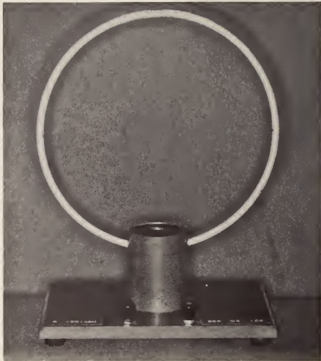
Figure 5.7. Standard Receiving Loop Used at 10 MHz.
