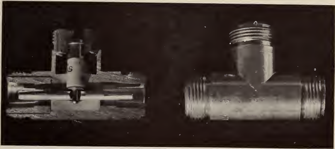
Figure 6.5. Cutaway of Diode Mount Used for Evaluating Frequency Response.
