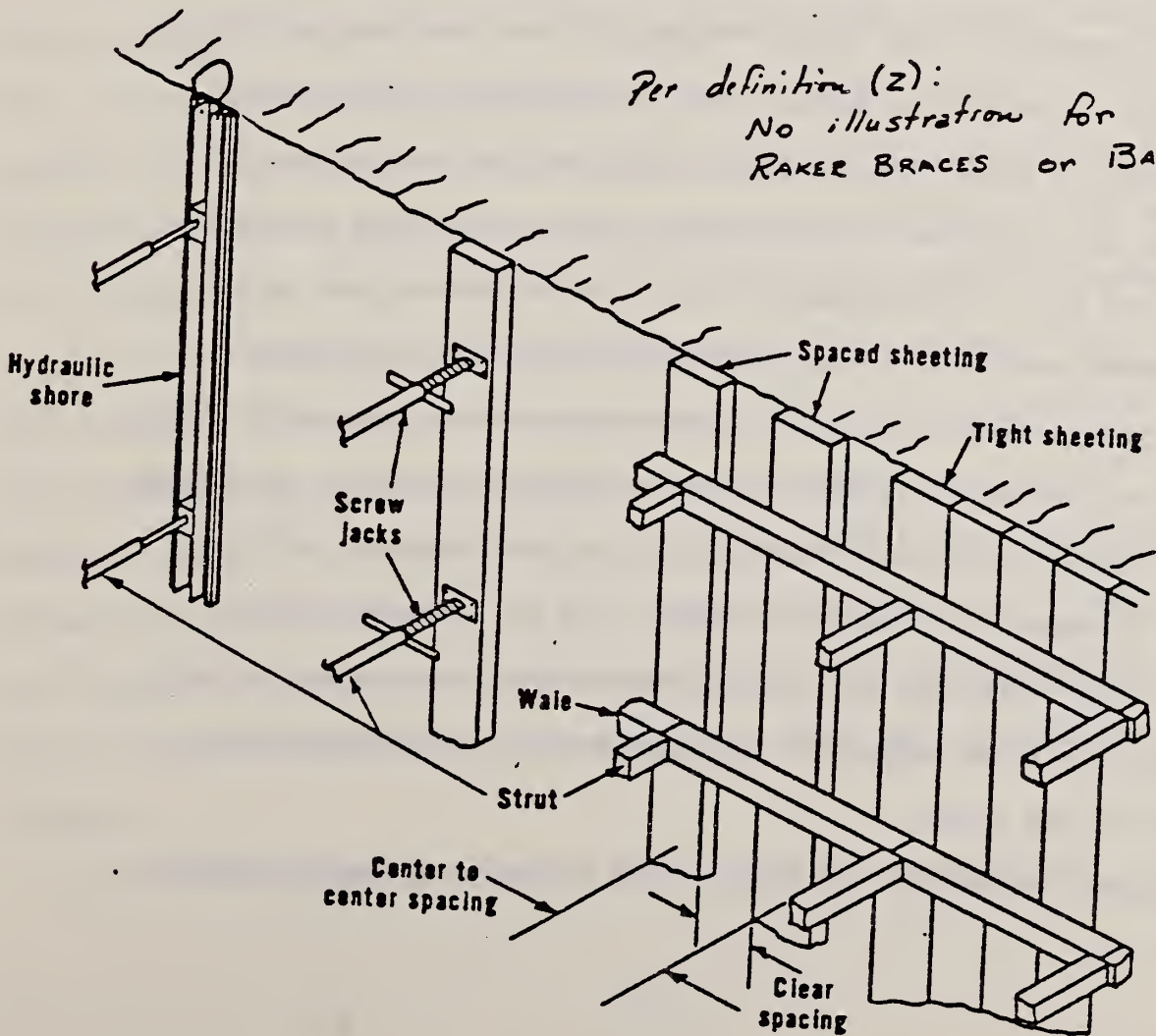
Figure 4. Components of the Shoring System
