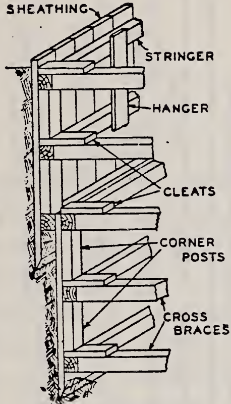
Fig. 2.—Trench Timbering—Loose Soil
